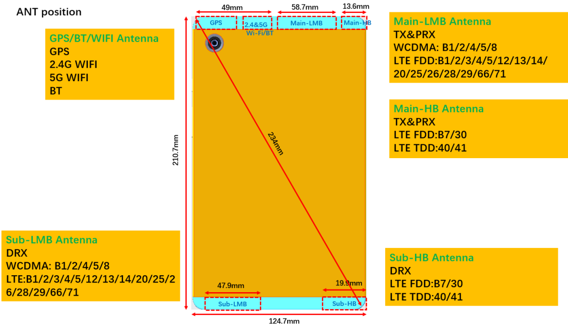
Picture 12 Antenna Locations
