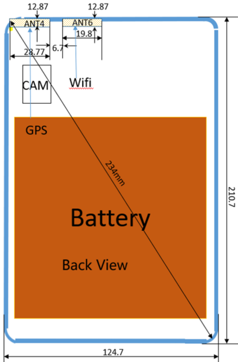
Picture 16: Antenna Locations
