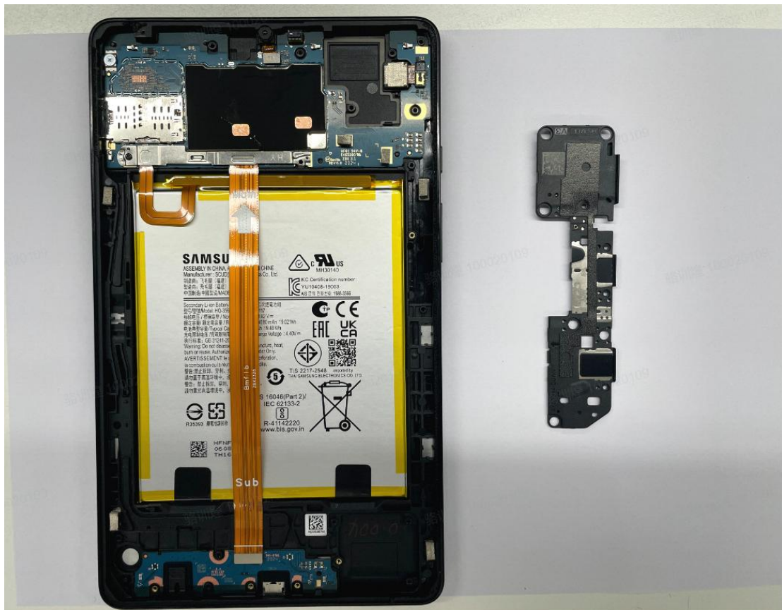
PCB05
