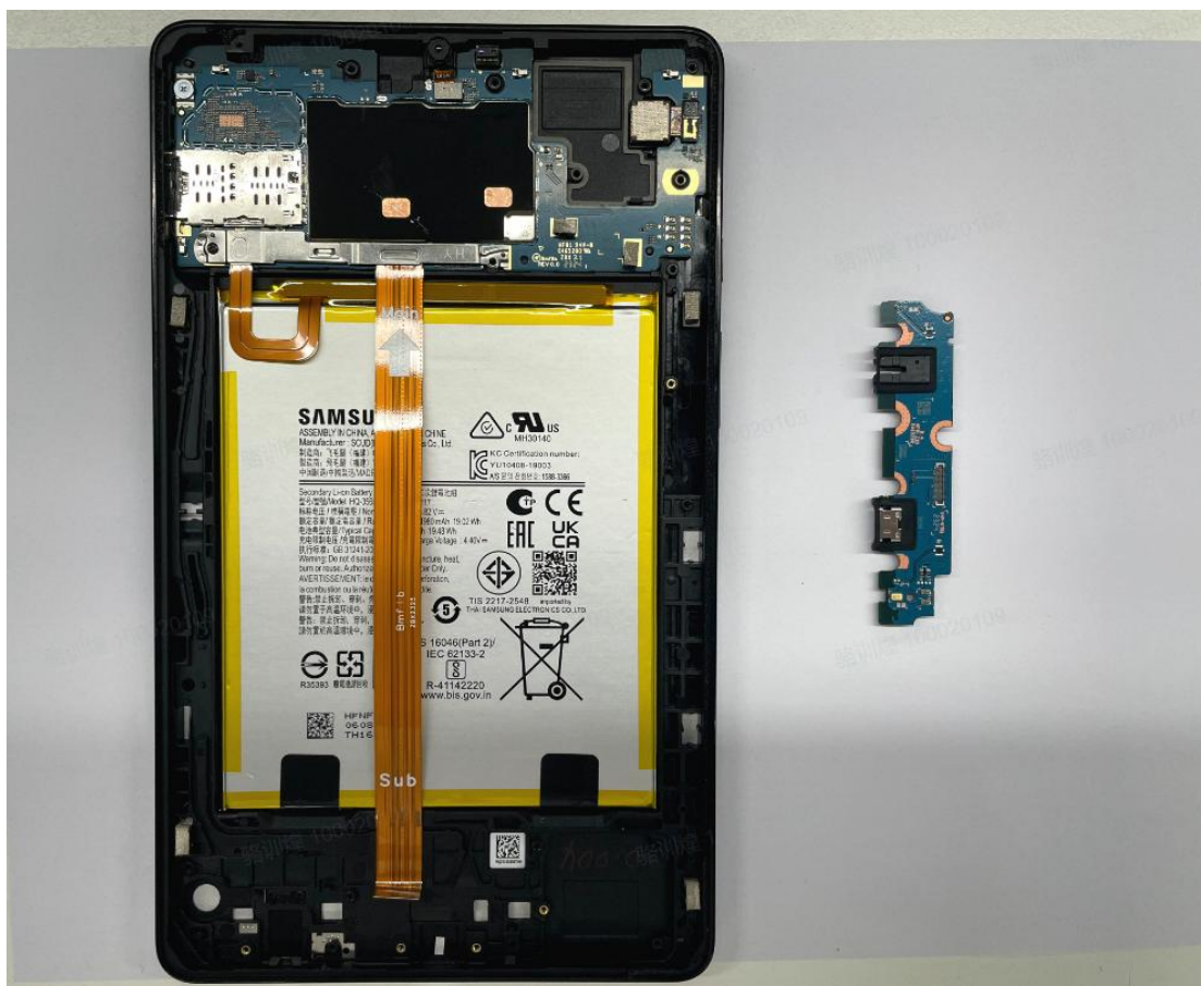
PCB06
