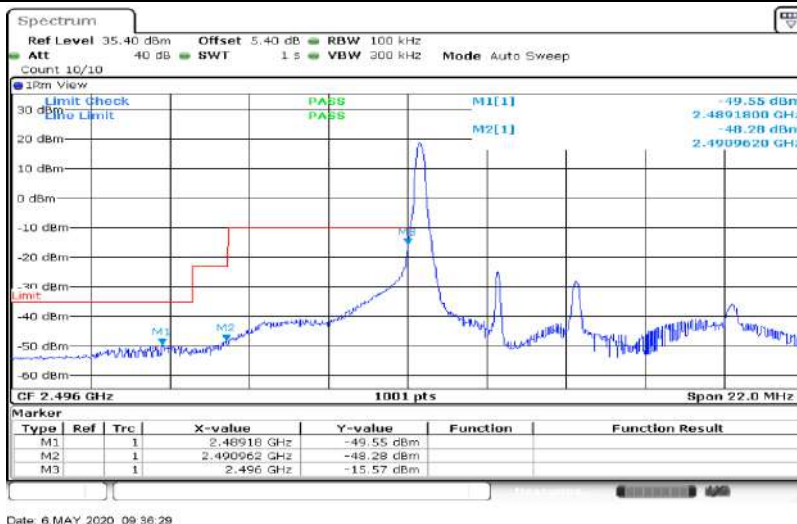
Band41-5MHz-16QAM-39675-25RB#0
