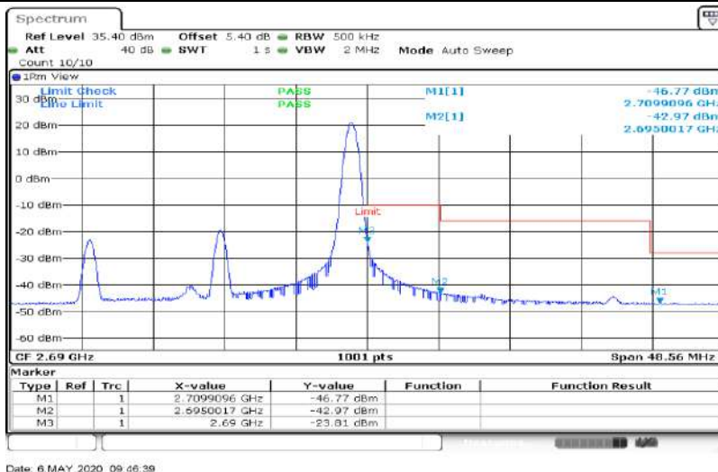
Band41-20MHz-16QAM-41490-100RB#0
