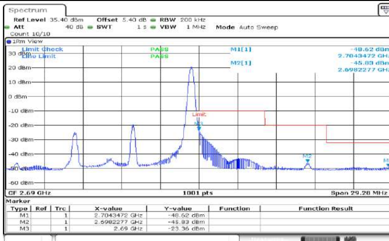
Band41-10MHz-16QAM-41540-1RB#49
