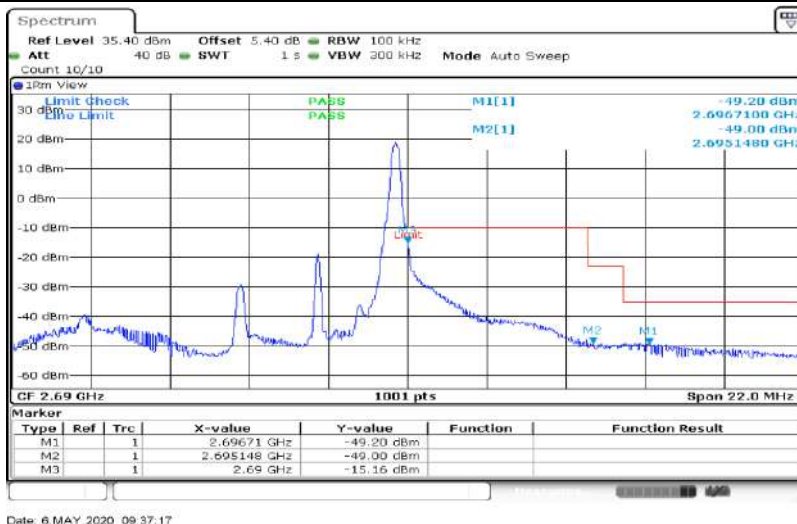
Band41-5MHz-16QAM-41565-25RB#0
