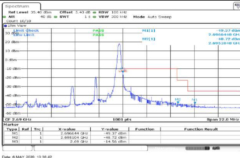
Band41-5MHz-64QAM-41565-25RB#0
