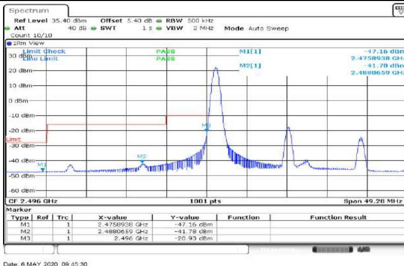
Band41-20MHz-QPSK-39750-100RB#0
