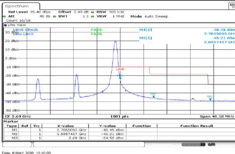
Band41-15MHz-64QAM-41515-75RB#0
