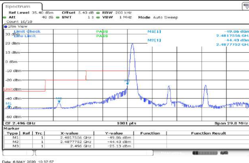
Band41-10MHz-64QAM-39700-50RB#0
