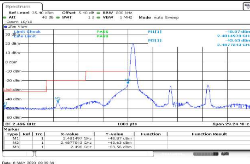
Band41-10MHz-16QAM-39700-50RB#0
