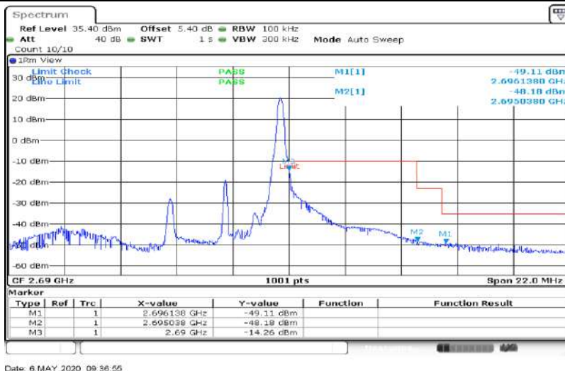
Band41-5MHz-QPSK-41565-25RB#0
