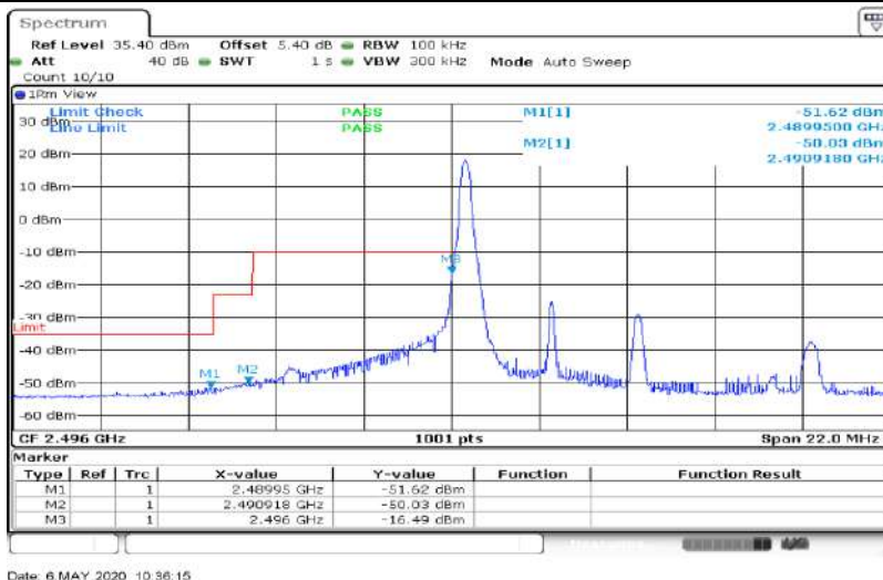
Band41-5MHz-64QAM-39675-25RB#0
