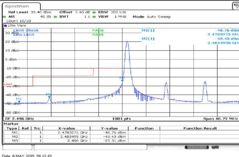
Band41-15MHz-16QAM-39725-75RB#0
