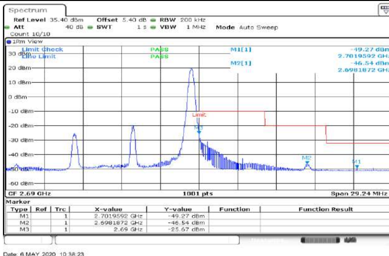
Band41-10MHz-64QAM-41540-50RB#0
