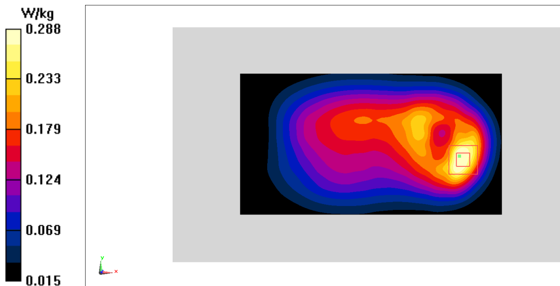
Fig.10 CDMA BC0
