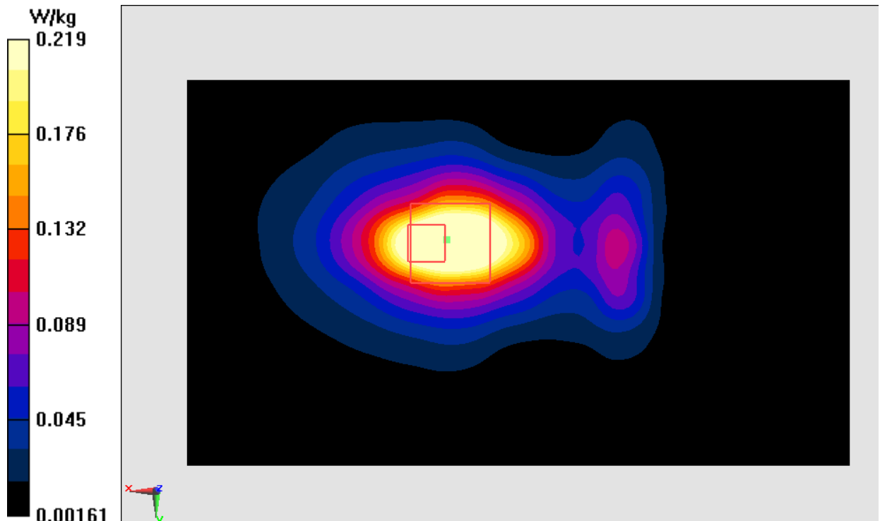
Fig.18 2450 MHz
