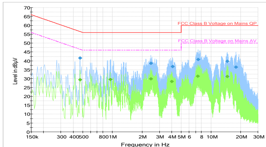
Figure B-12: Measurement results for Conducted Emission
