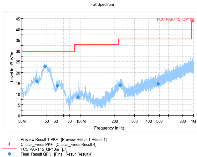
Figure B-7: Measurement results for Electric Field Radiated Emissions (≥30MHz)
