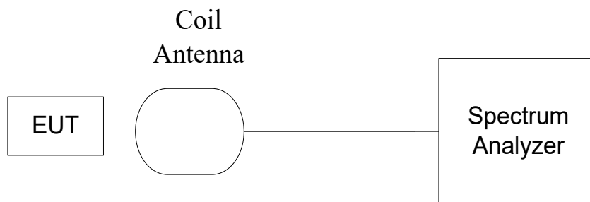
Figure B-9: Measurement Setup
