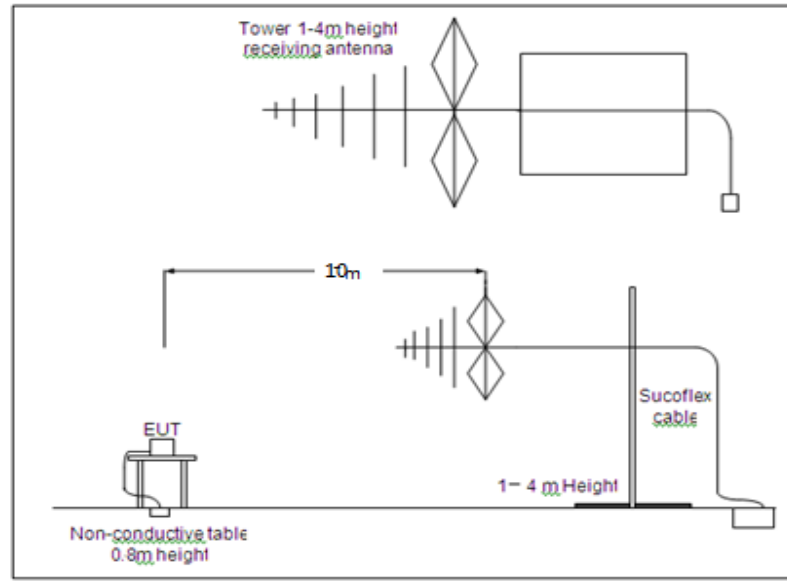
Figure B-6: Measurement Setup
