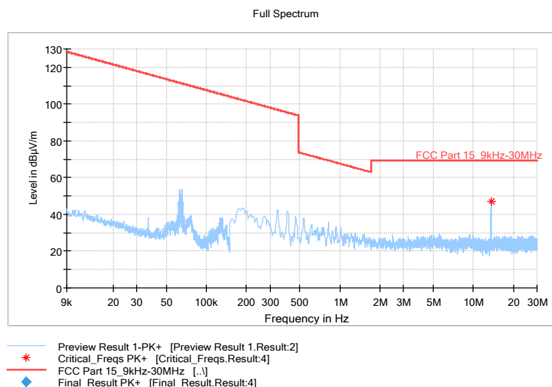
Figure B-5: Measurement results for Electric Field Radiated Emissions (< 30MHz)
