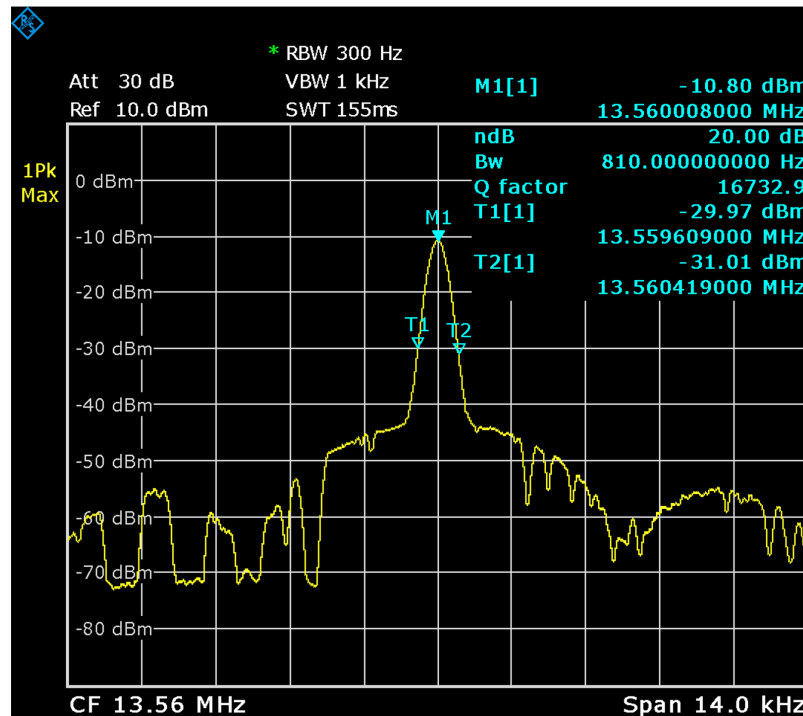
Figure B-10: Measurement results for 20dB Bandwidth
