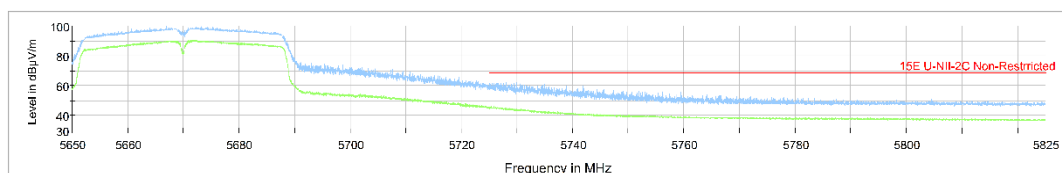
Fig.49 Band Edges (802.11ac-HT40 Ch134, 5670MHz)
