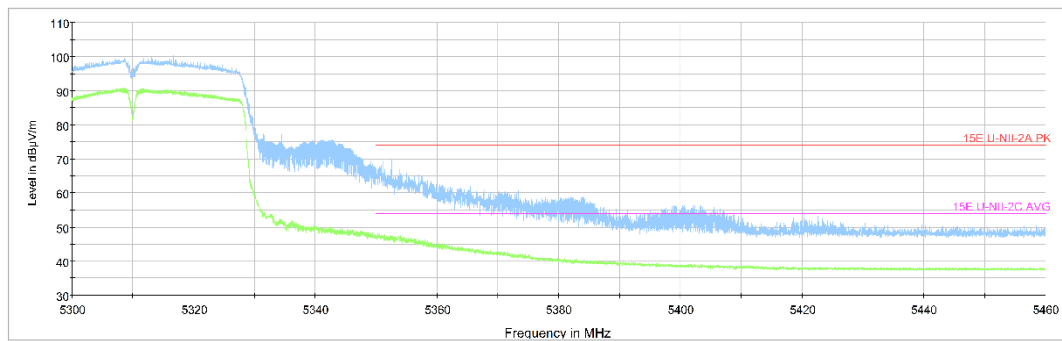
Fig.39 Band Edges (802.11n-HT40 Ch62, 5310MHz)
