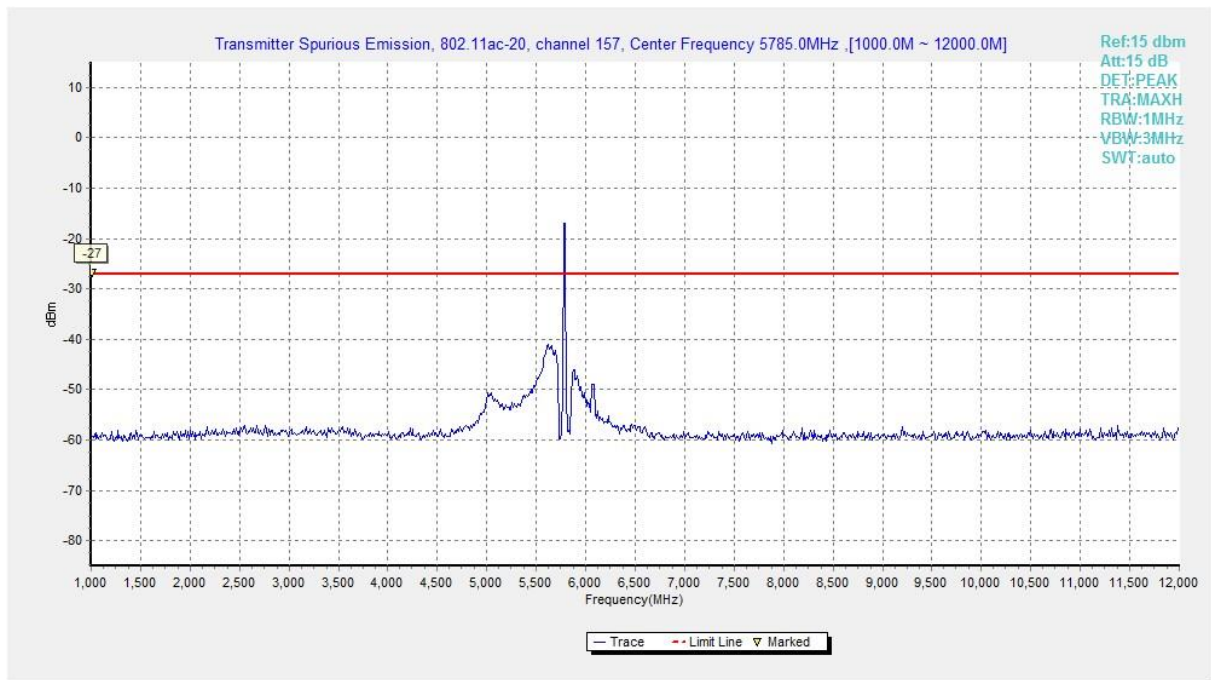
Fig. 44 Conducted Spurious Emission (802.11ac20, Ch157 , 1 GHz ~ 12 GHz)
