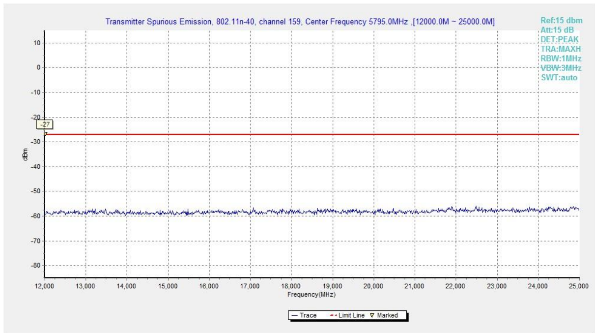
Fig. 57 Conducted Spurious Emission (802.11n40, Ch159 , 12 GHz ~ 25 GHz)
