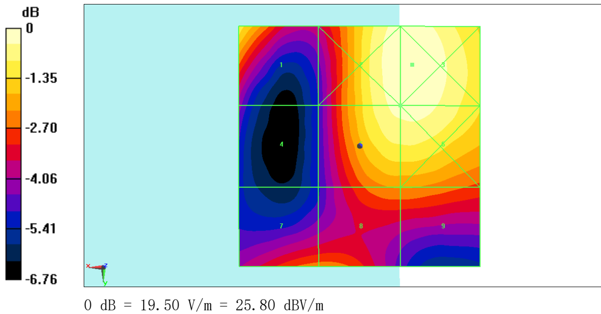
Fig B.7 HAC RF E-Field LTE Band41 Power Class 3 16QAM CH39750
