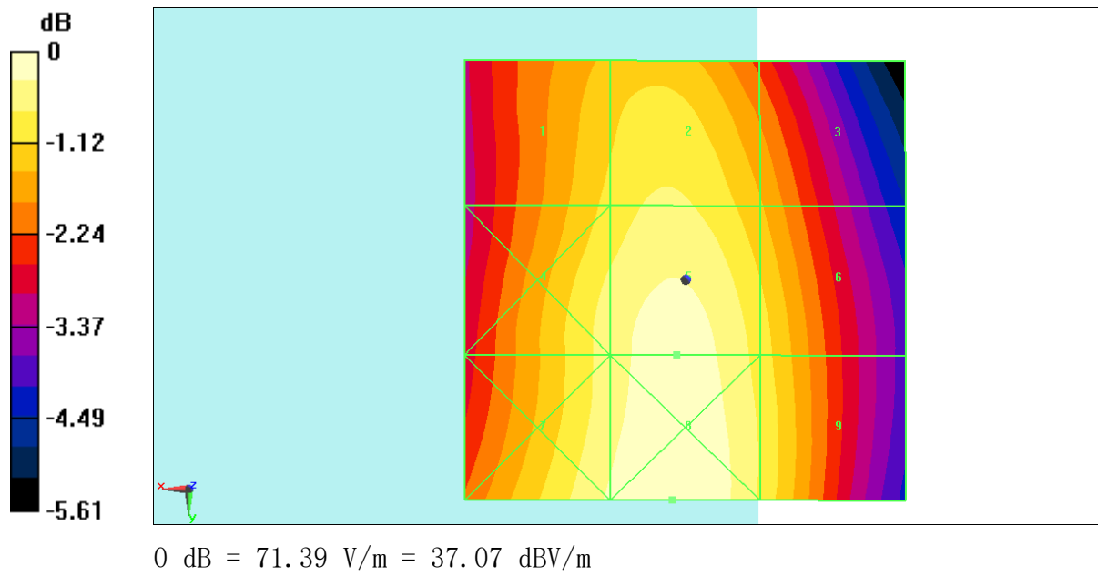
Fig B.1 HAC RF E-Field GSM 850 Middle
