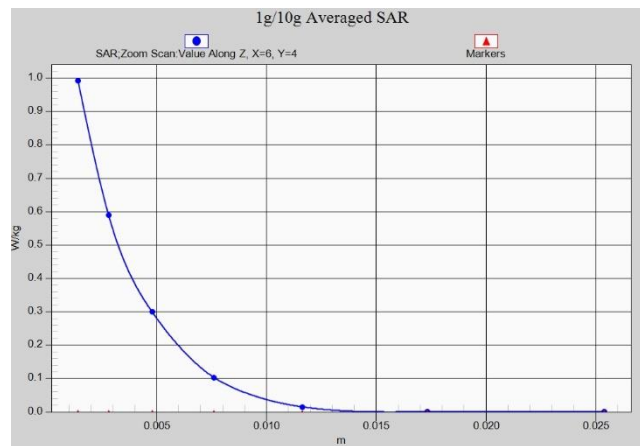
Fig. 1-31 Z-Scan at power reference point (5 GHz)
