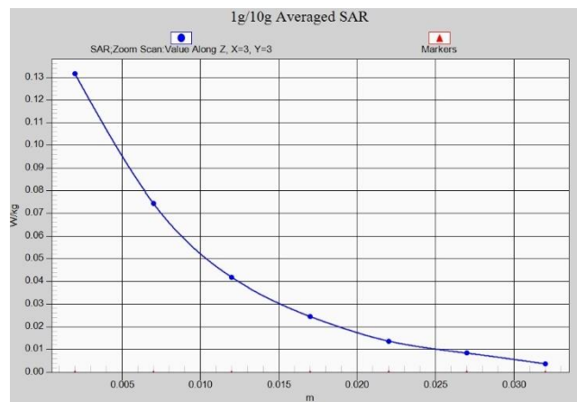
Fig. 1-23 Z-Scan at power reference point (LTE Band41-PC2)
