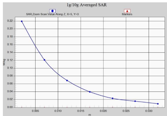
Fig. 1-21 Z-Scan at power reference point (LTE Band41-PC3)
