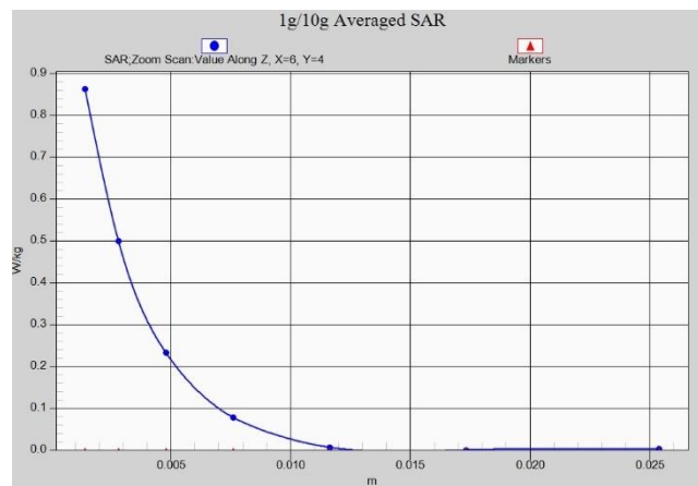
Fig. 1-32 Z-Scan at power reference point (5 GHz)
