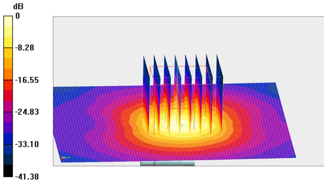
Fig.B.17 validation 5750 MHz 100mW
