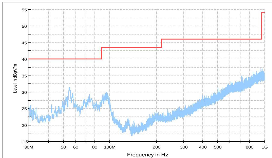
Figure A.63 Radiated Emission from 30MHz to 1GHz
