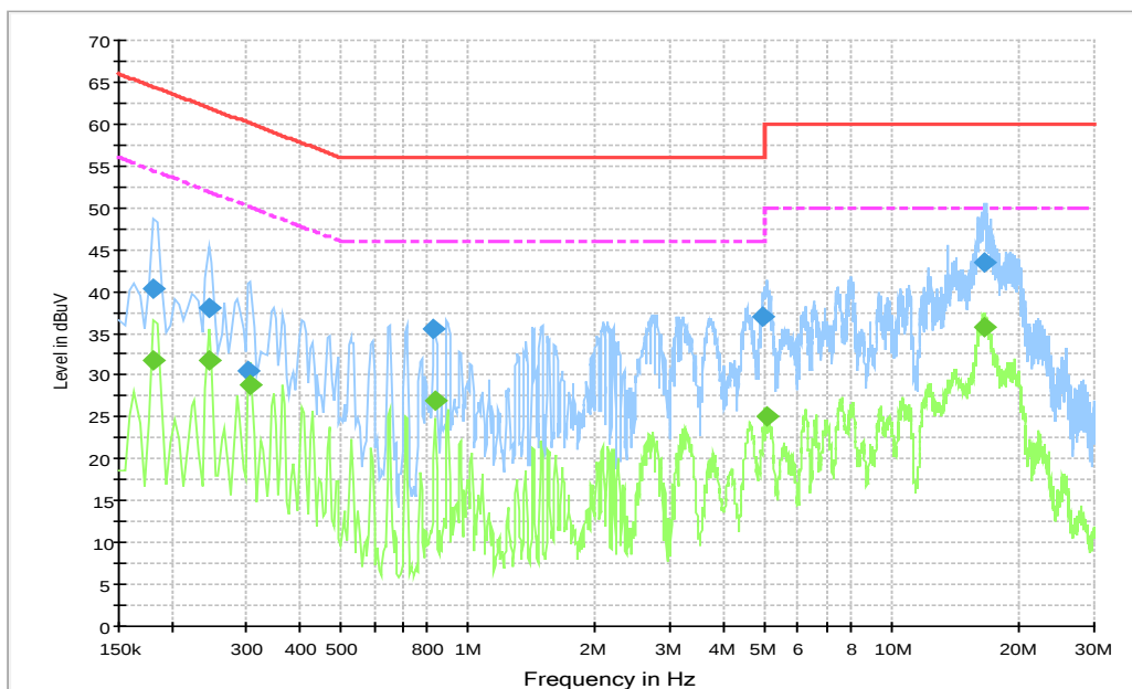
Figure A.73 Conducted Emission
