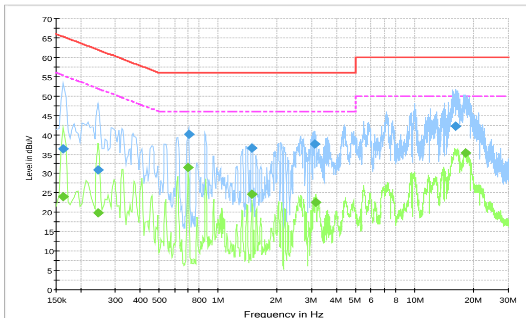
Figure A.72 Conducted Emission
