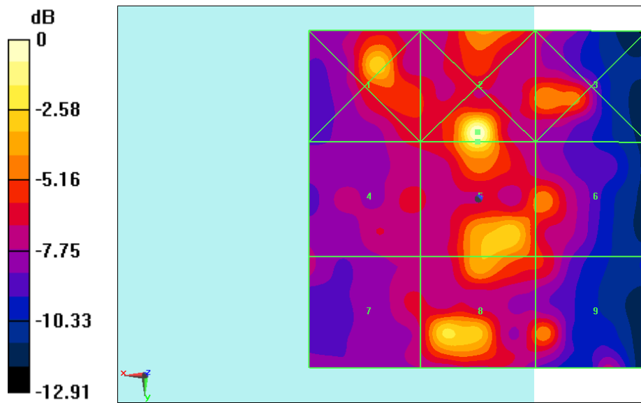
Fig B.3 HAC RF E-Field CDMA BC0 Low
