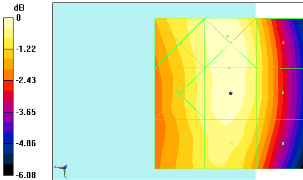
Fig B.5 HAC RF E-Field CDMA BC10 High
