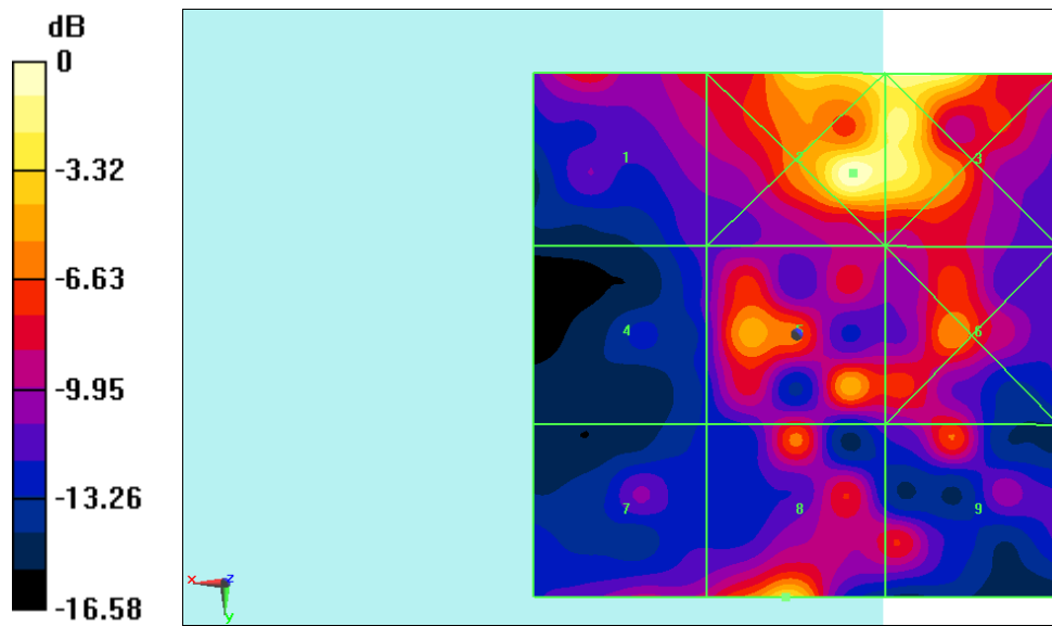
Fig B.4 HAC RF E-Field CDMA BC1 High
