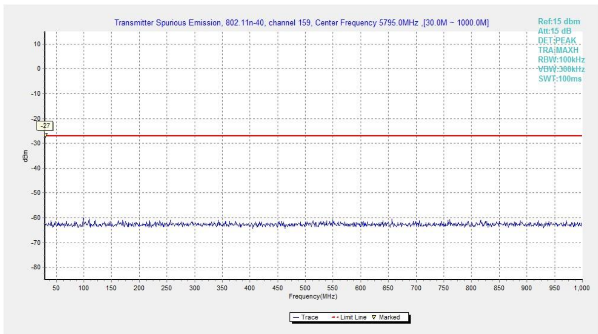
Fig. 55 Conducted Spurious Emission (802.11n40, Ch159 , 30 MHz ~ 1 GHz)
