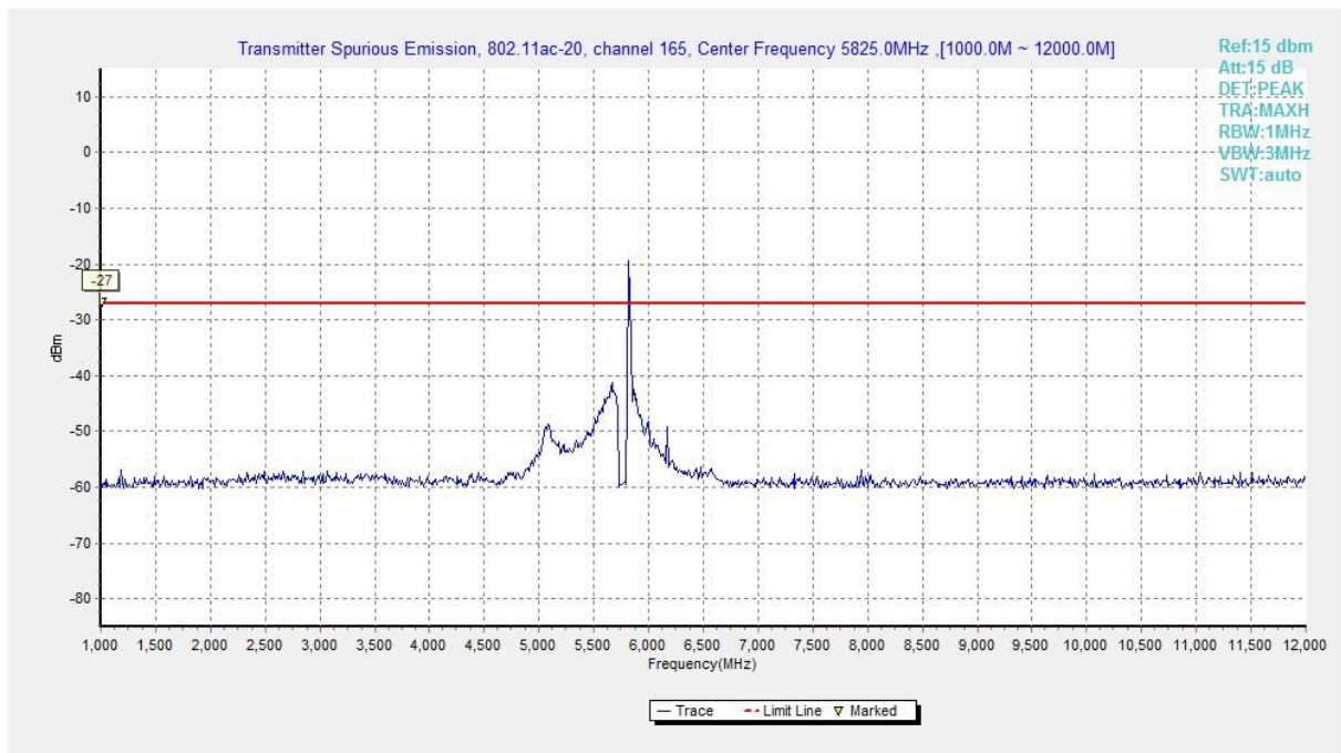
Fig. 48 Conducted Spurious Emission (802.11ac20, Ch165 , 1 GHz ~ 12 GHz)
