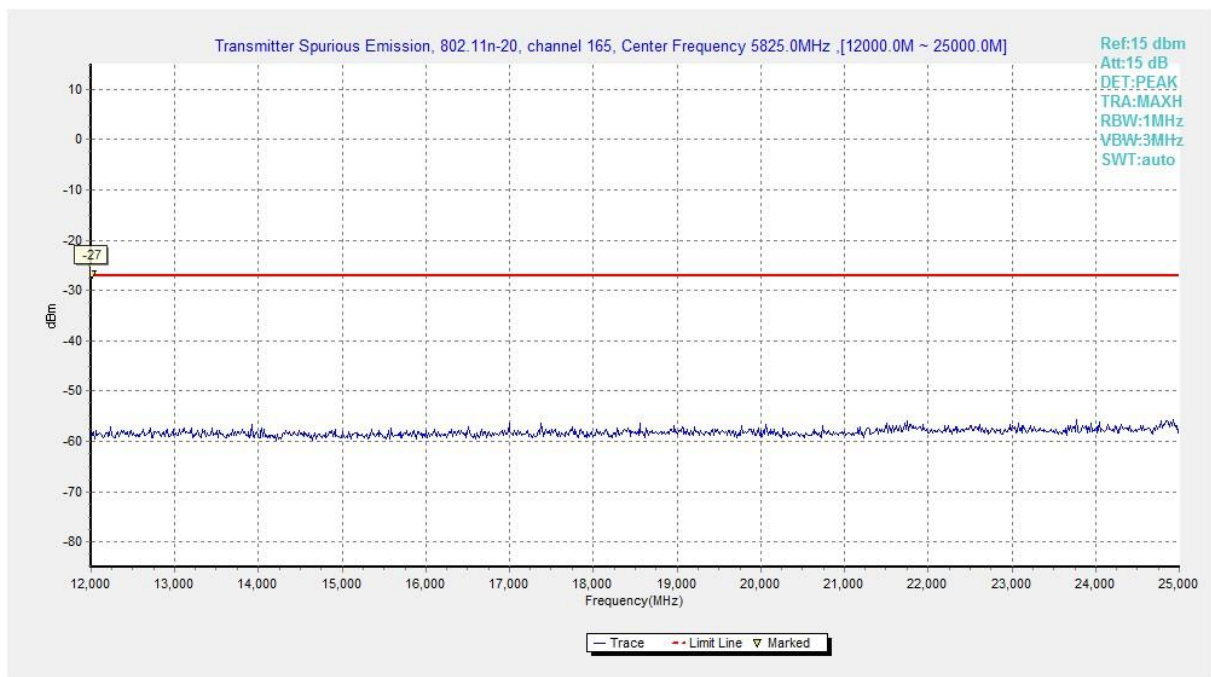
Fig. 37 Conducted Spurious Emission (802.11n20, Ch165 , 12 GHz ~ 25 GHz)
