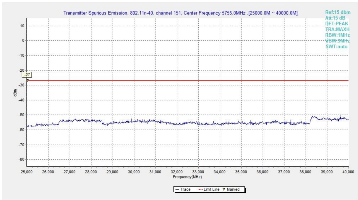
Fig. 54 Conducted Spurious Emission (802.11n40, Ch151 , 25 GHz ~ 40 GHz)
