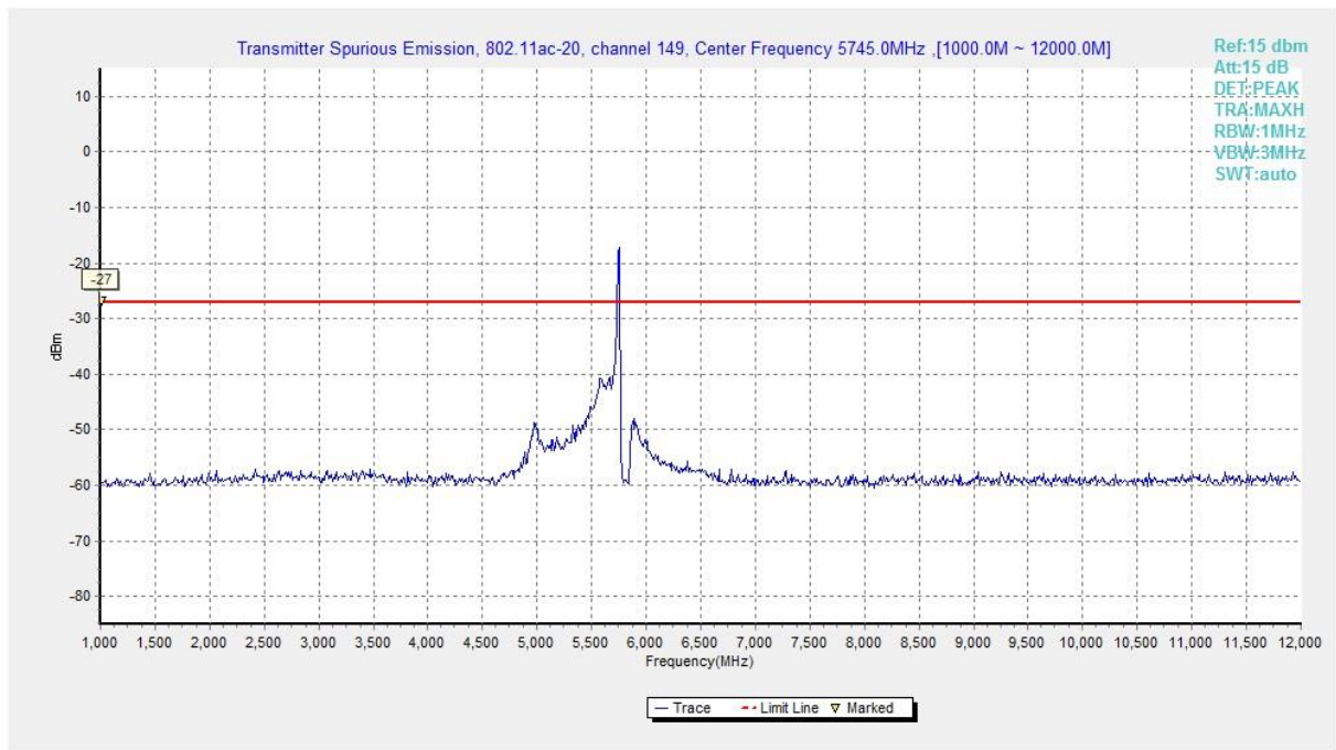
Fig. 40 Conducted Spurious Emission (802.11ac20, Ch149 , 1 GHz ~ 12 GHz)
