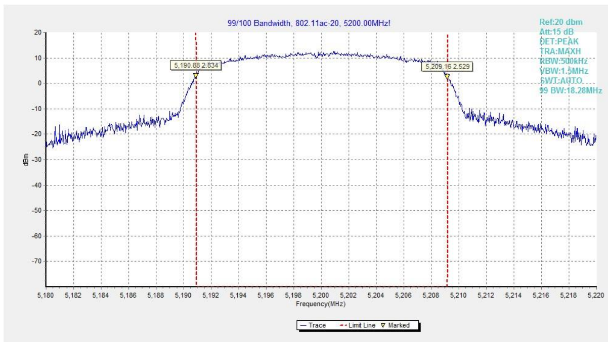
Fig.97 99% Occupied bandwidth (802.11ac-HT20, 5200MHz)
