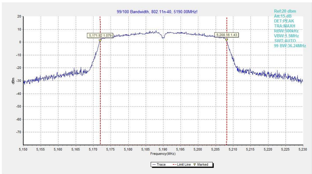
Fig.99 99% Occupied bandwidth (802.11n-HT40, 5190MHz)
