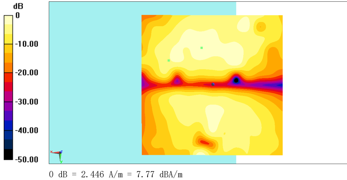
Fig B.9 T-Coil WiFi-5G
