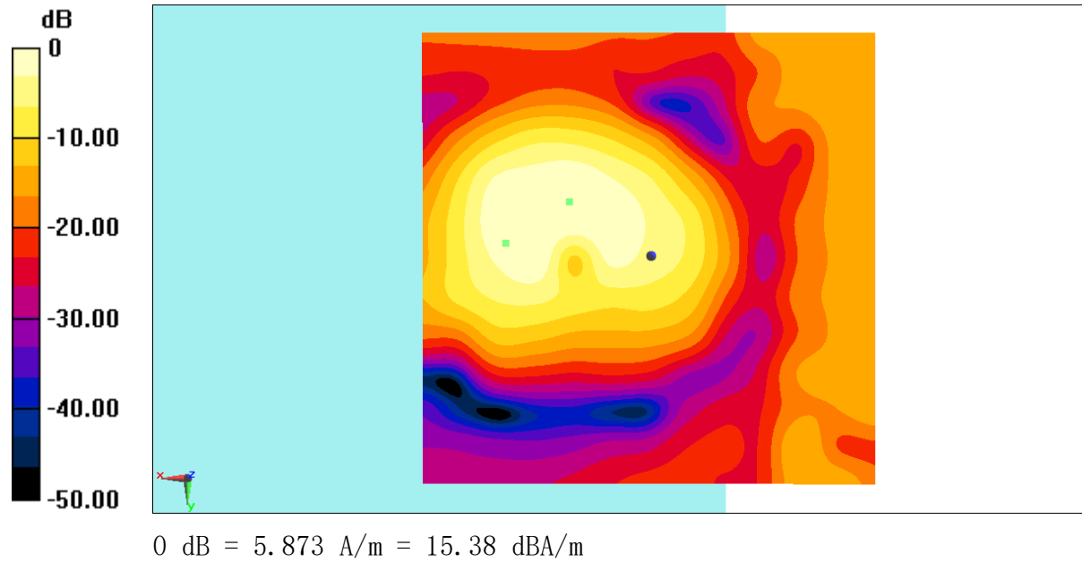
Fig B.10 T-Coil WiFi-5G
