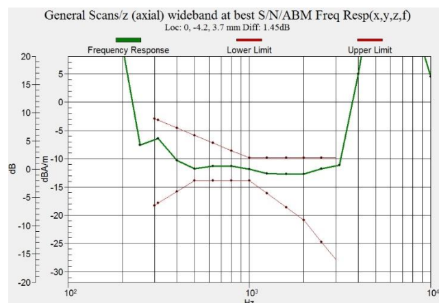
Figure C.3 Frequency Response of LTE B12
