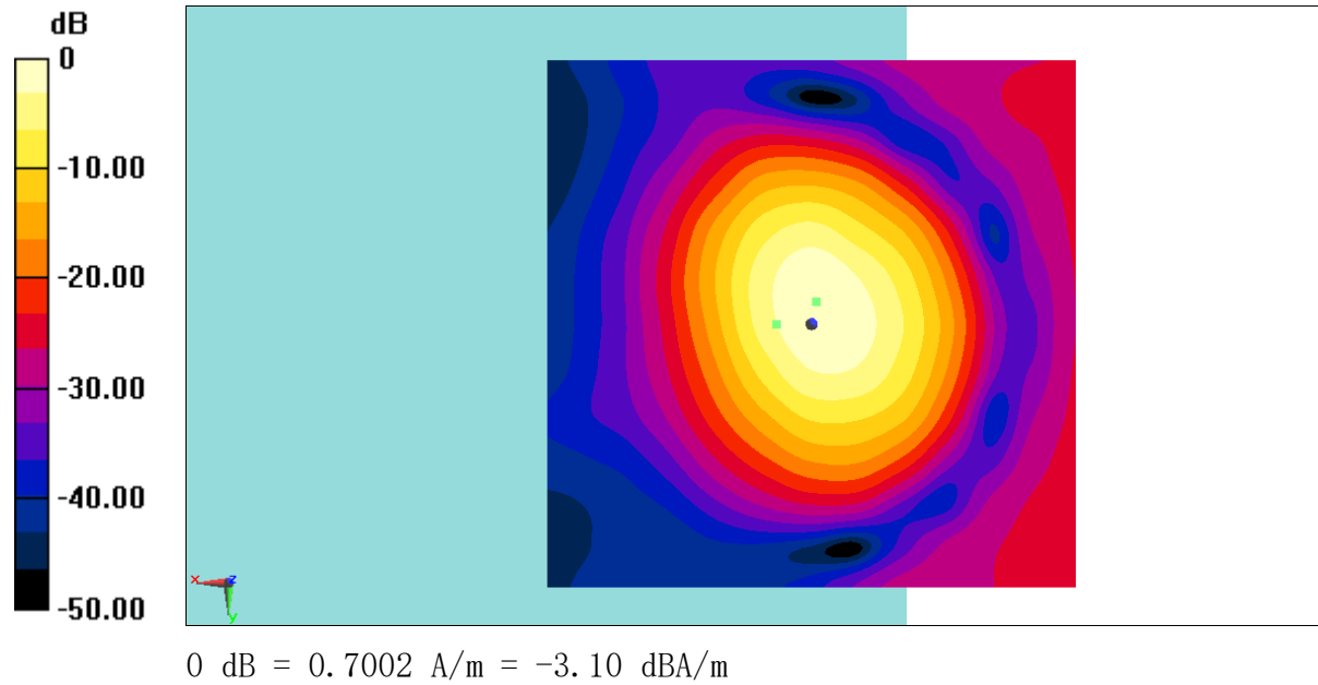
Fig B.6 T-Coil LTE B12
