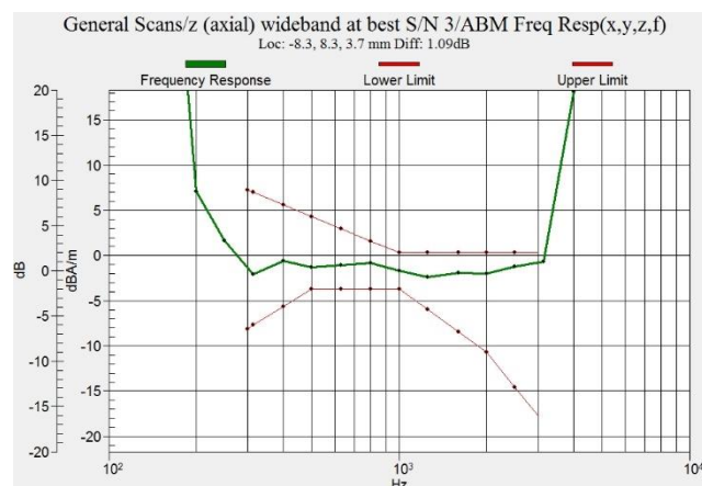
Figure C.9 Frequency Response of WiFi-5G - OTT VoIP
