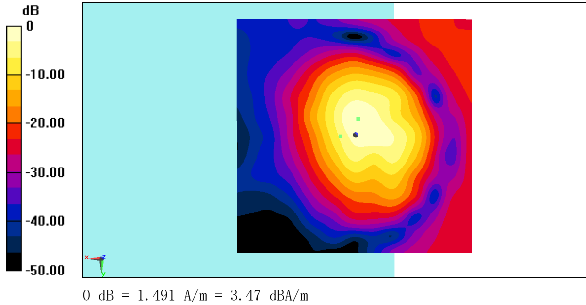
Fig B.14 T-Coil LTE B7
