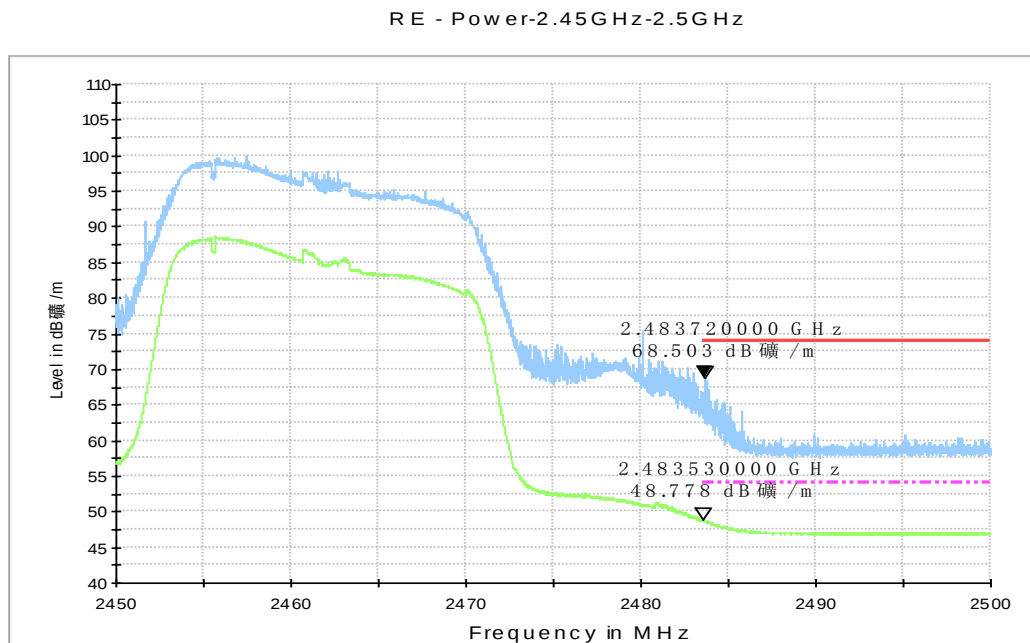
Fig.A.6.2.8 Transmitter Spurious Emission - Radiated (Power): 802.11n-HT20, ch11, 2.45 GHz - 2.50GHz
