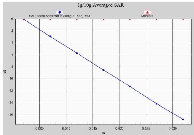
Fig. 20-1 Z-Scan at power reference point (2450 MHz)
