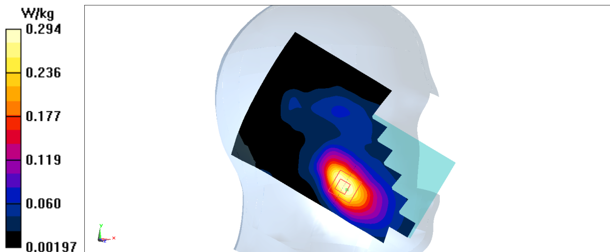
Fig.9 LTE Band2
