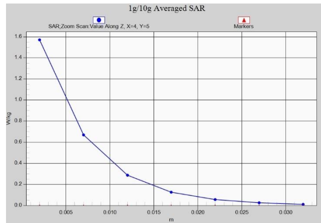
Fig. 19-1 Z-Scan at power reference point (2450 MHz)
