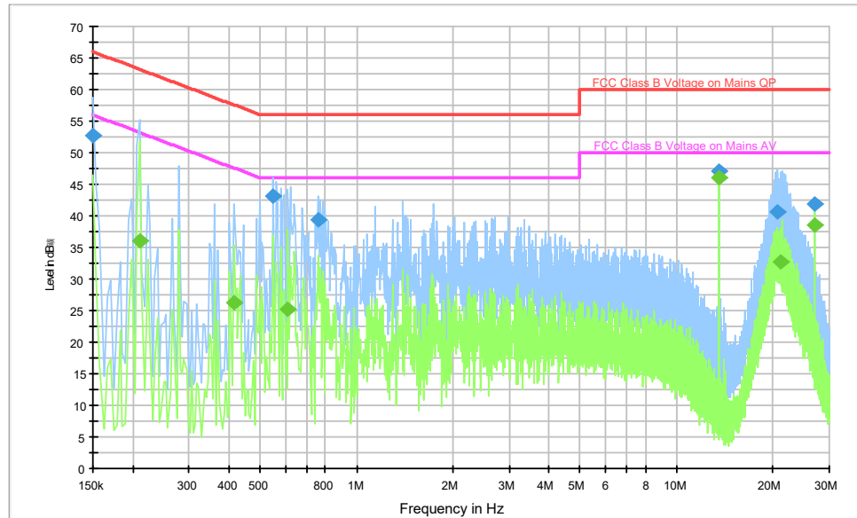
Figure B-11: Measurement results for Conducted Emission
