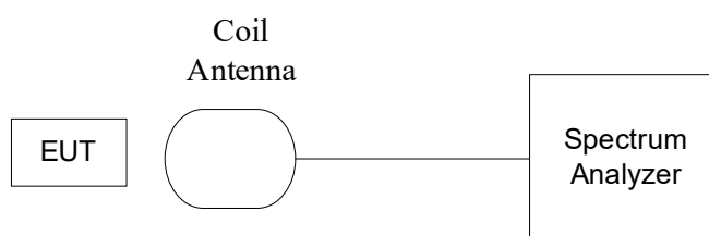
Figure B-8: Measurement Setup
