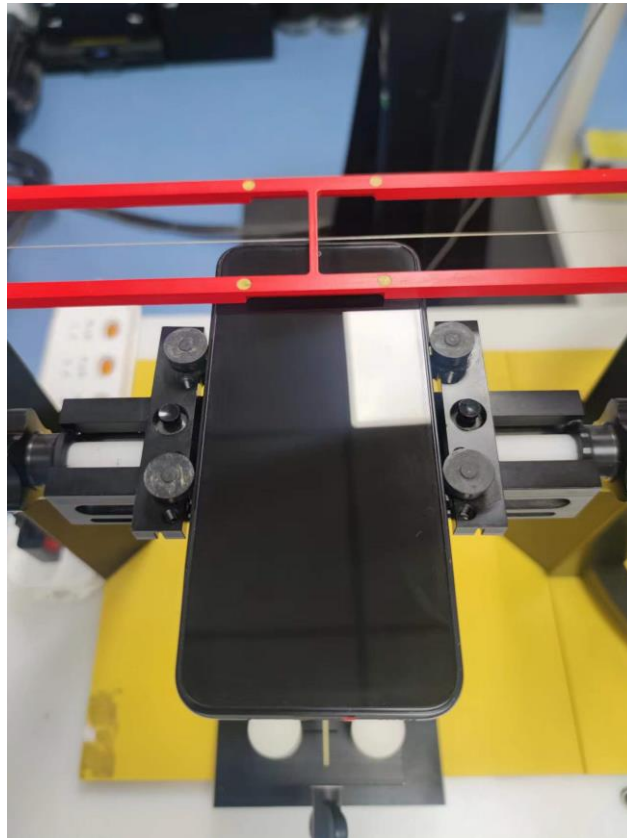
Picture 2: EUT Positioning for RF/T-coil
