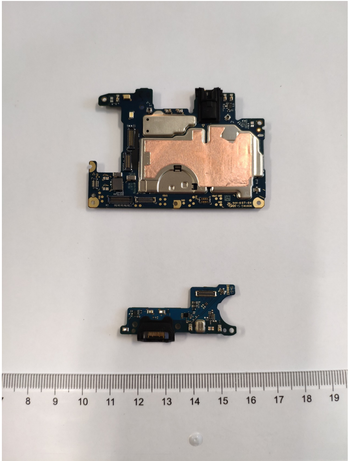
PCB05:
