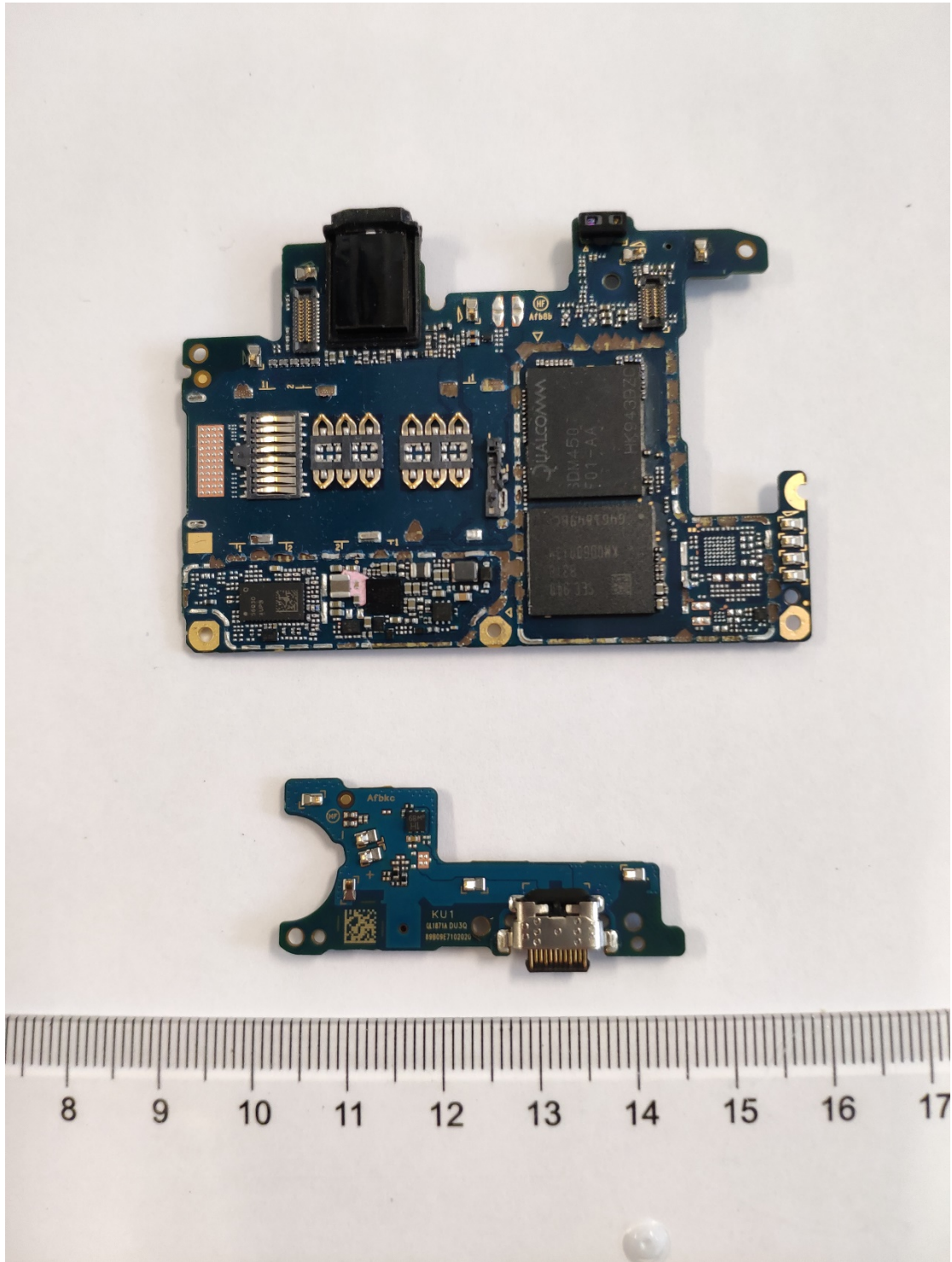
PCB07:
