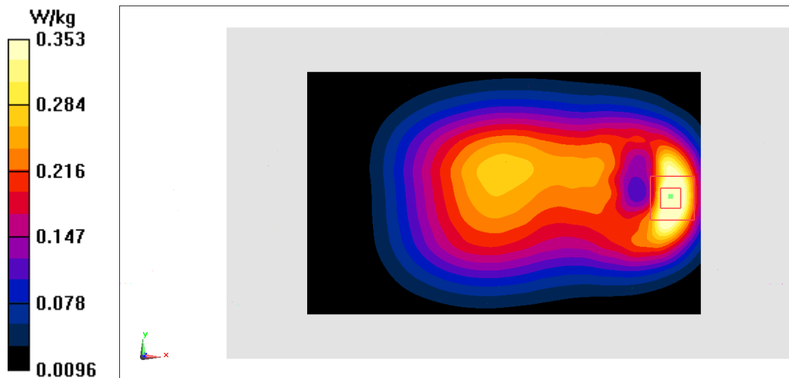
Fig.2 GSM850
