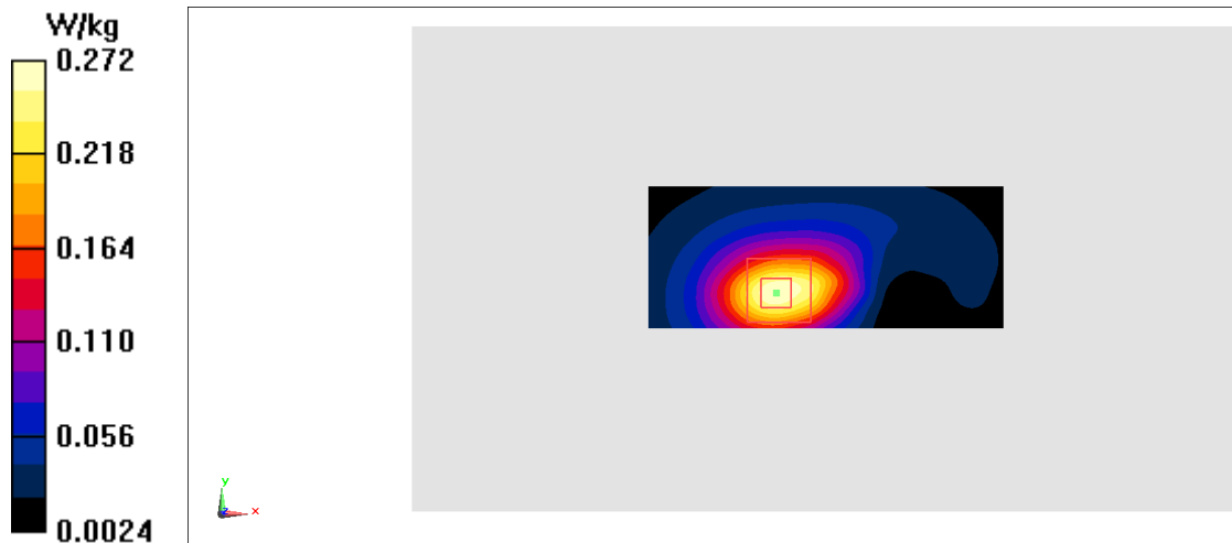
Fig.12 LTE Band 41
