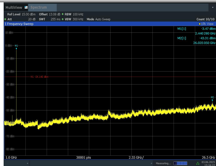
BLE_1M_Ant1_2440_1000~26500
