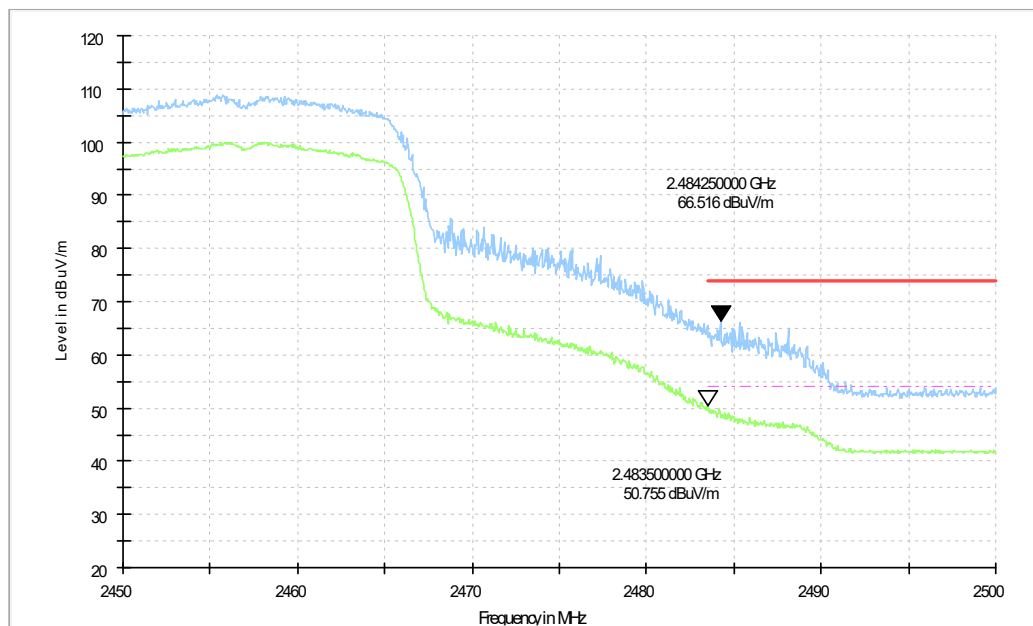
Fig.13 Transmitter Spurious Emission - Radiated (Power): 802.11n-HT20, ch10, 2.45 GHz - 2.50GHz
