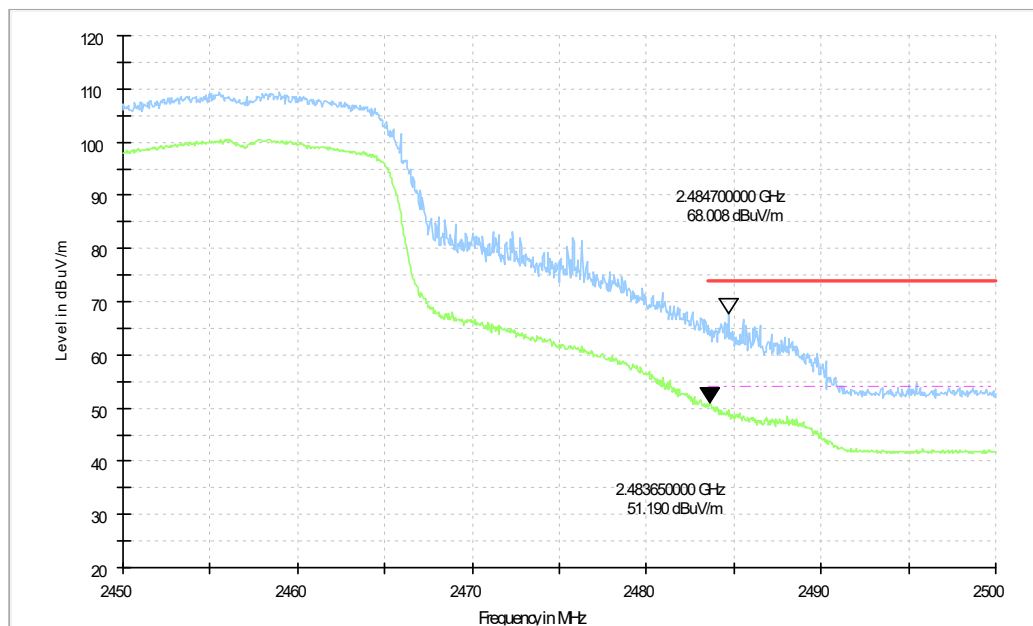
Fig.7 Transmitter Spurious Emission - Radiated (Power): 802.11g, ch10, 2.45 GHz - 2.50GHz
