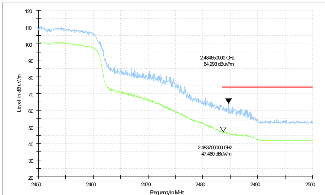
Fig.12 Transmitter Spurious Emission - Radiated (Power): 802.11n-HT20, ch9, 2.45 GHz - 2.50GHz
