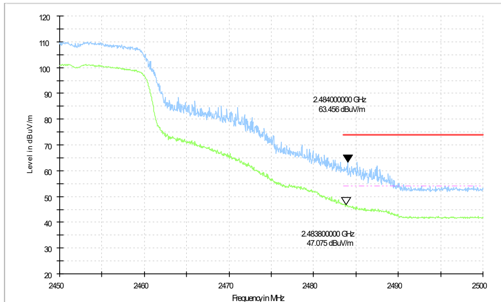
Fig.6 Transmitter Spurious Emission - Radiated (Power): 802.11g, ch9, 2.45 GHz - 2.50GHz
