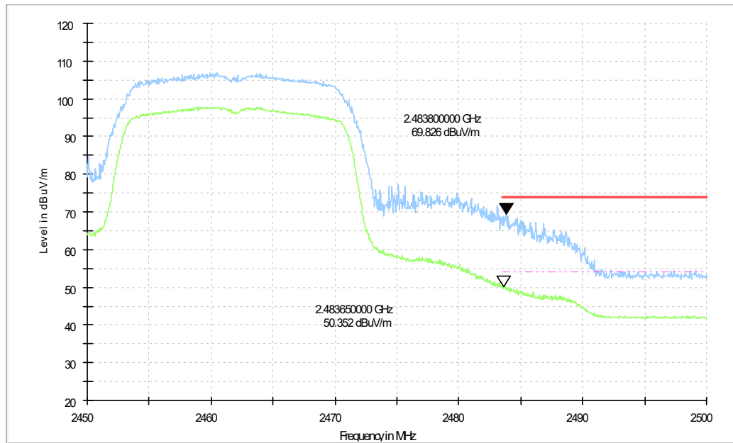
Fig.14 Transmitter Spurious Emission - Radiated (Power): 802.11n-HT20, ch11, 2.45 GHz - 2.50GHz
