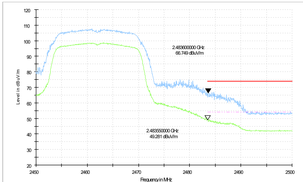
Fig.8 Transmitter Spurious Emission - Radiated (Power): 802.11g, ch11, 2.45 GHz - 2.50GHz
