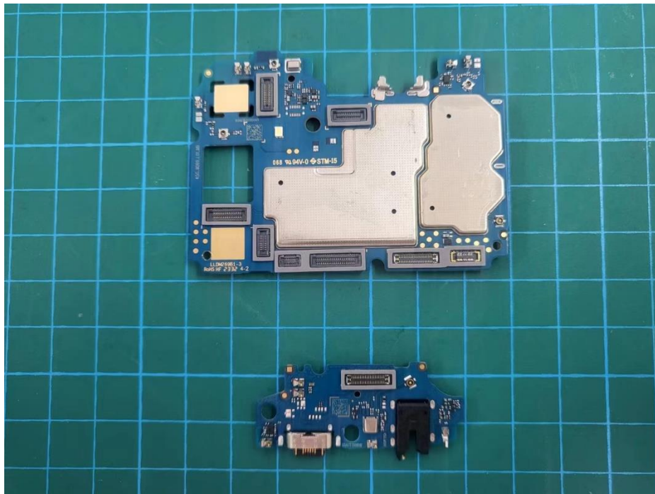
PCB04
