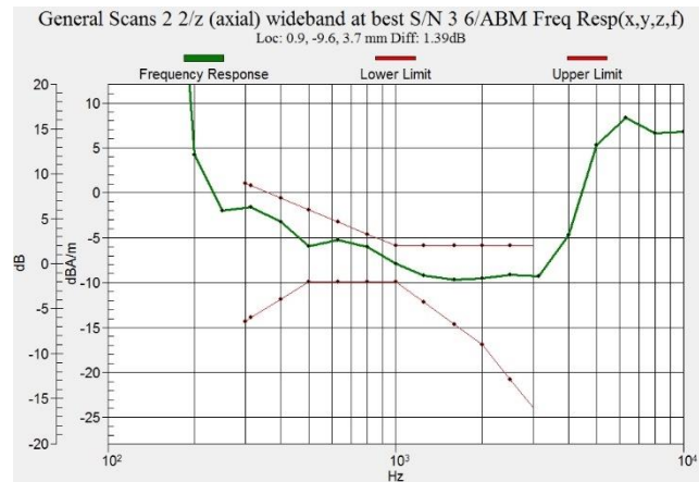
Figure C.2 Frequency Response of LTE B5
