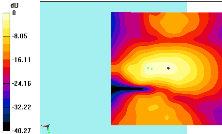
Fig B.3 T-Coil LTE B5
