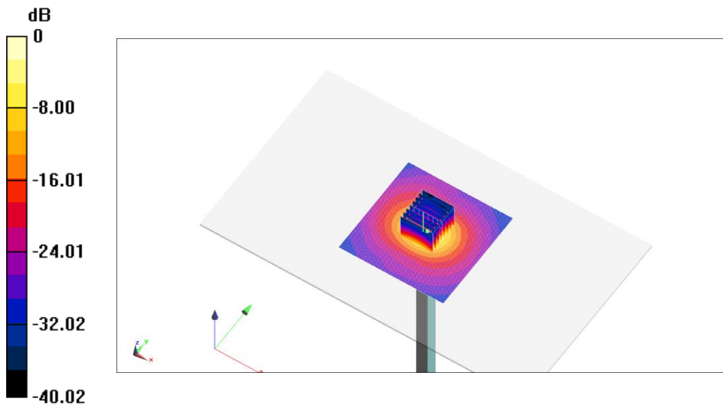
Fig.B.6 validation 5250 MHz 250mW
