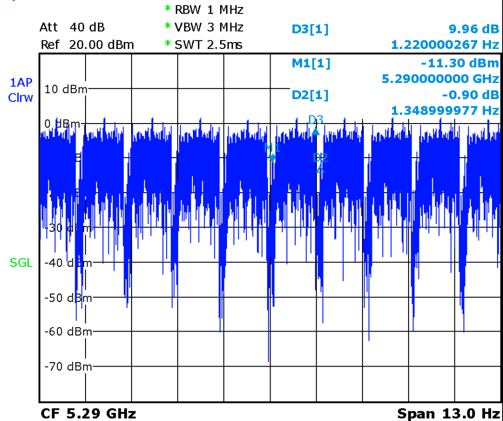
Picture 14.4 The plot of duty factor-Low Power
