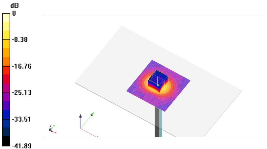
Fig.B.7 validation 5600 MHz 250mW
