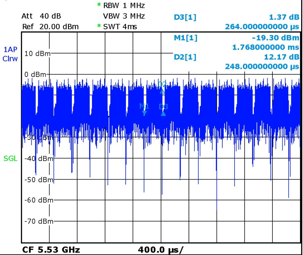
Picture 14.5 The plot of duty factor-Normal Power
