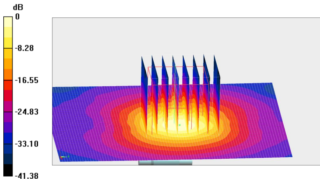
Fig.B.8 validation 5750 MHz 250mW
