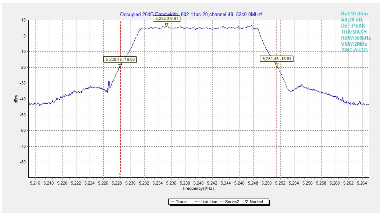
Fig.13 Occupied 26dB Bandwidth (802.11ac-HT20, 5240MHz)
