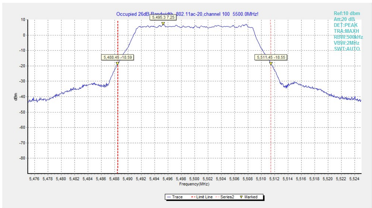
Fig.17 Occupied 26dB Bandwidth (802.11ac-HT20, 5500MHz)
