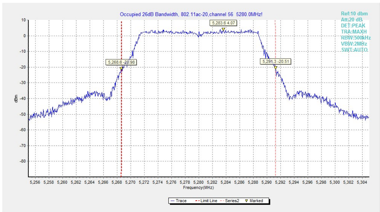
Fig.15 Occupied 26dB Bandwidth (802.11ac-HT20, 5280MHz)
