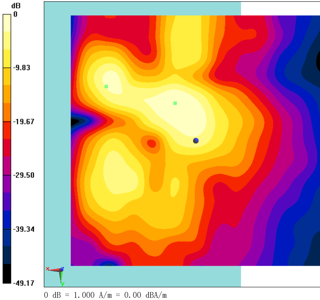
Fig B.29 T-Coil WiFi-5G
