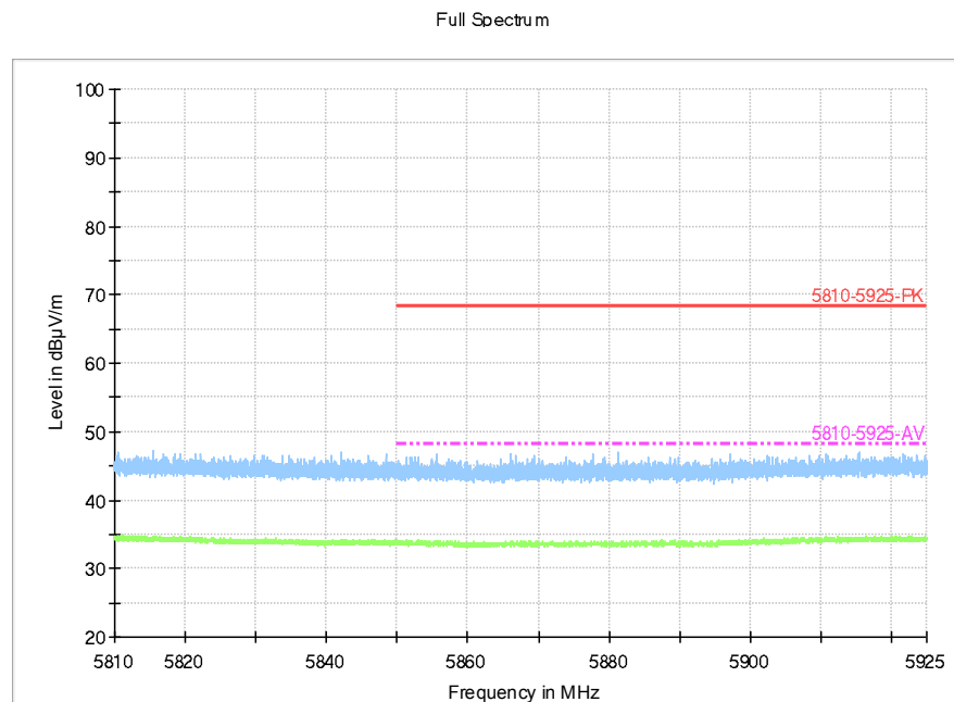
Fig.33 Band Edges (802.11a, 5720MHz)
