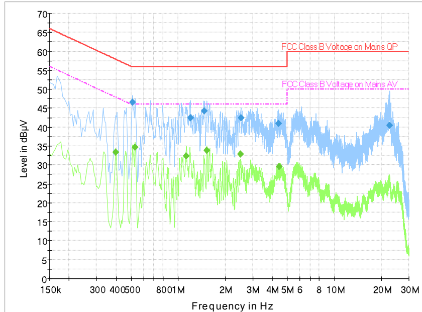
Fig.48 Conducted Emission(802.11a, IDLE)
