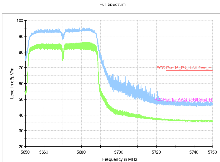
Fig.44 Band Edges (802.11n-HT40, 5670MHz)
