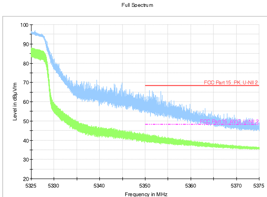
Fig.42 Band Edges (802.11n-HT40, 5310MHz)
