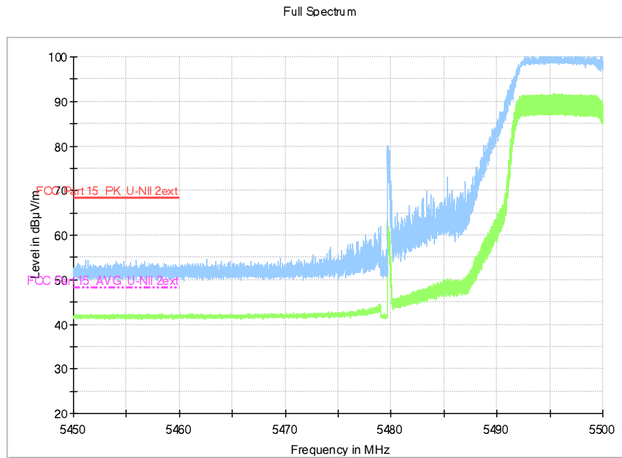
Fig.31 Band Edges (802.11a, 5500MHz)
