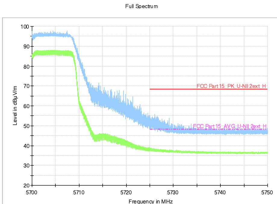
Fig.38 Band Edges (802.11n-HT20, 5700MHz)
