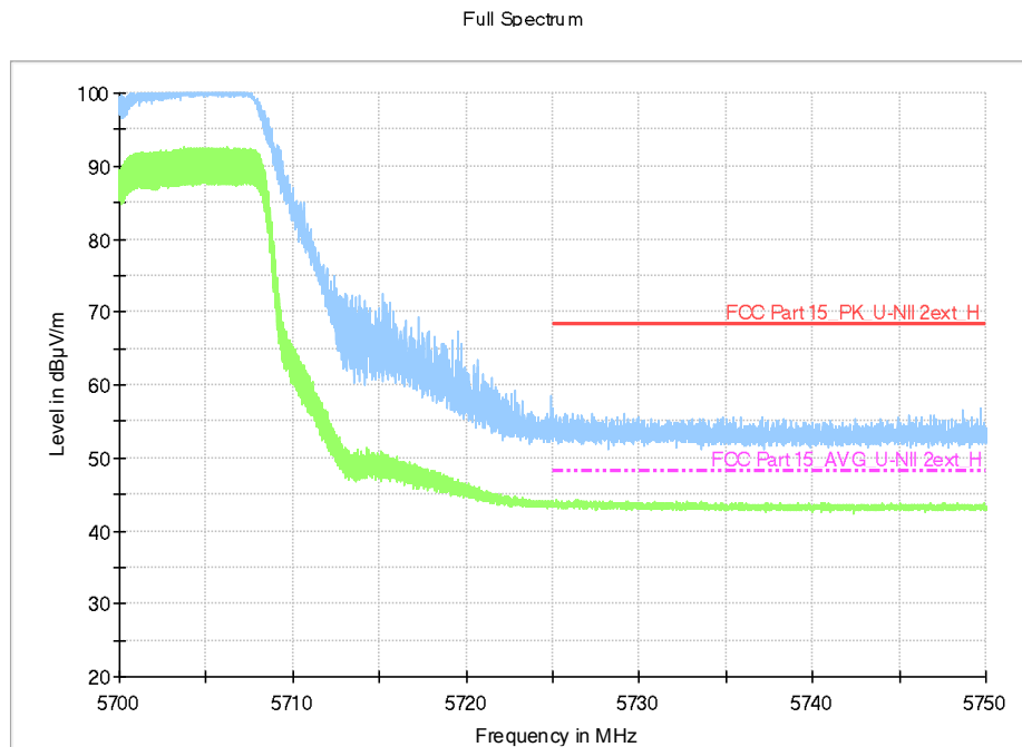
Fig.32 Band Edges (802.11a, 5700MHz)
