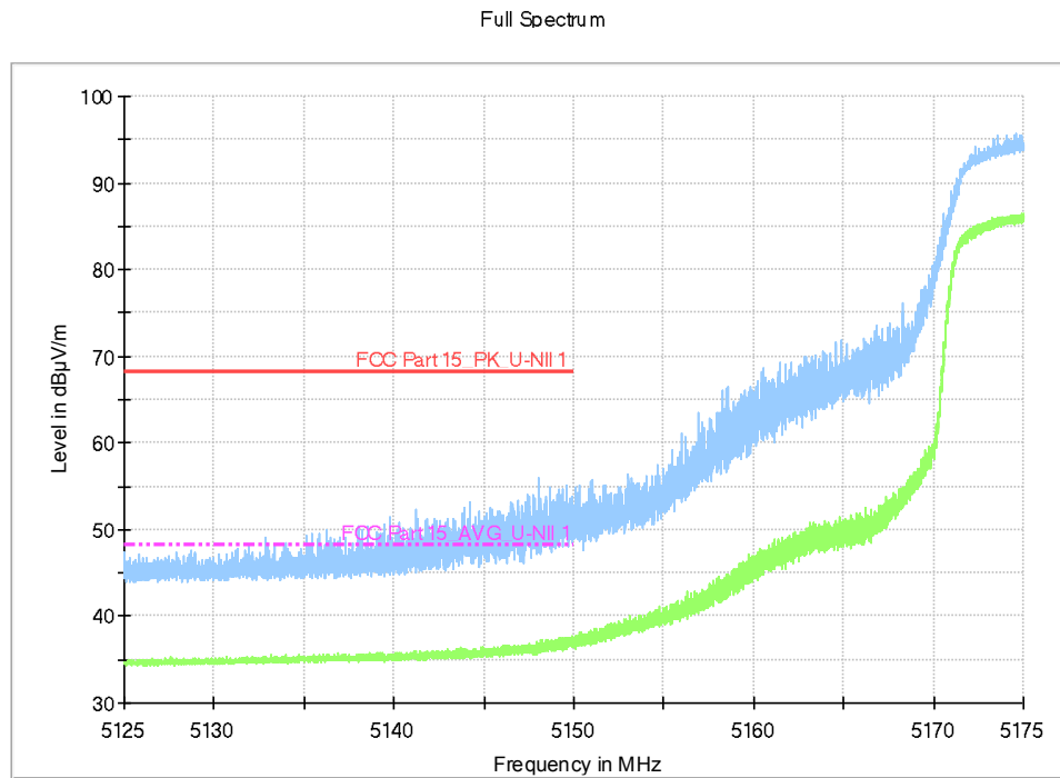
Fig.41 Band Edges (802.11n-HT40, 5190MHz)
