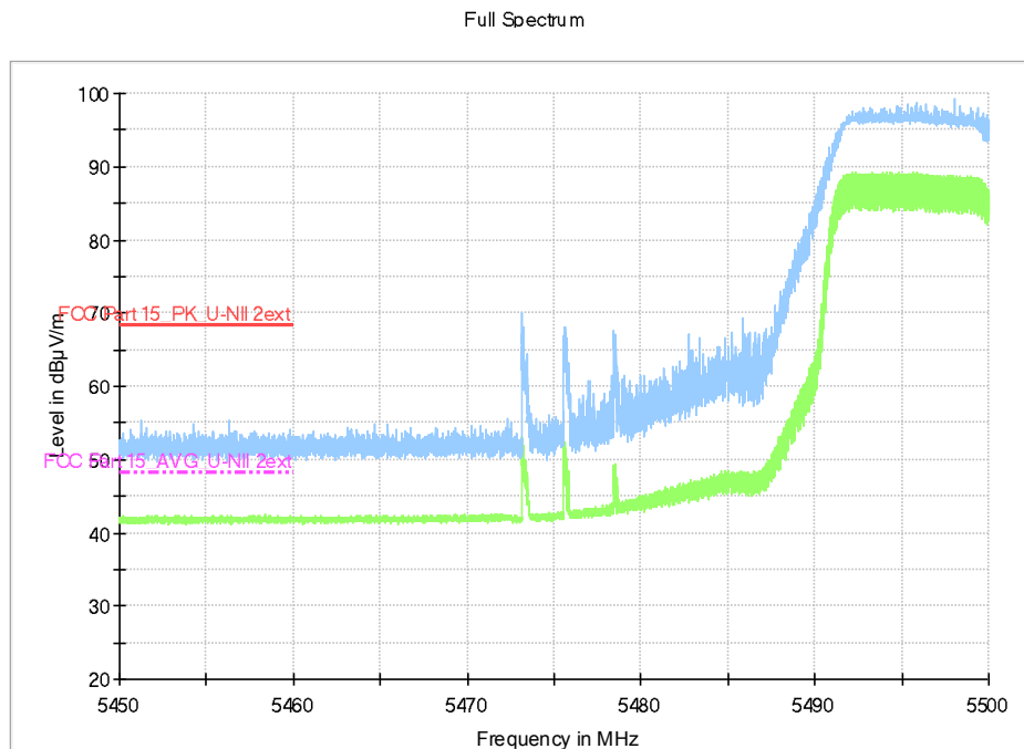
Fig.37 Band Edges (802.11n-HT20, 5500MHz)
