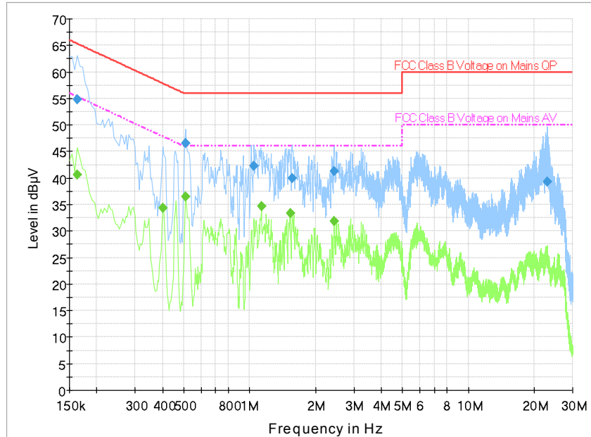
Fig.47 Conducted Emission(802.11a, Ch40, TX)
