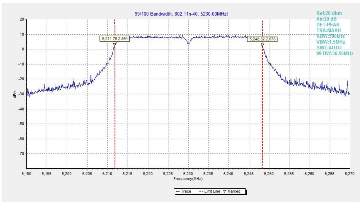
Fig.56 99% Occupied bandwidth (802.11n-HT40, 5230MHz)
