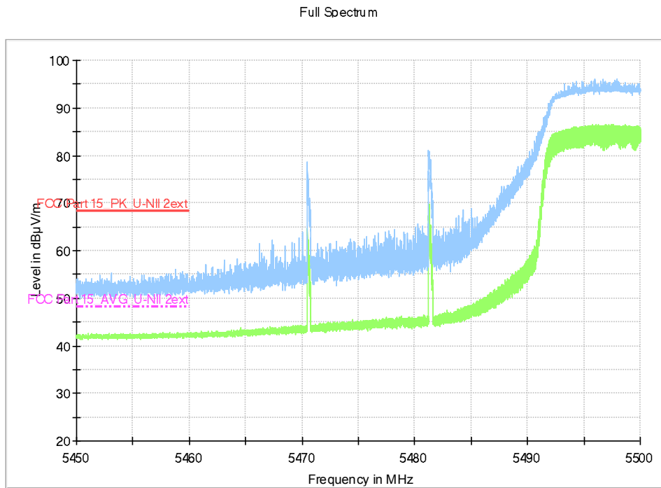
Fig.43 Band Edges (802.11n-HT40, 5510MHz)
