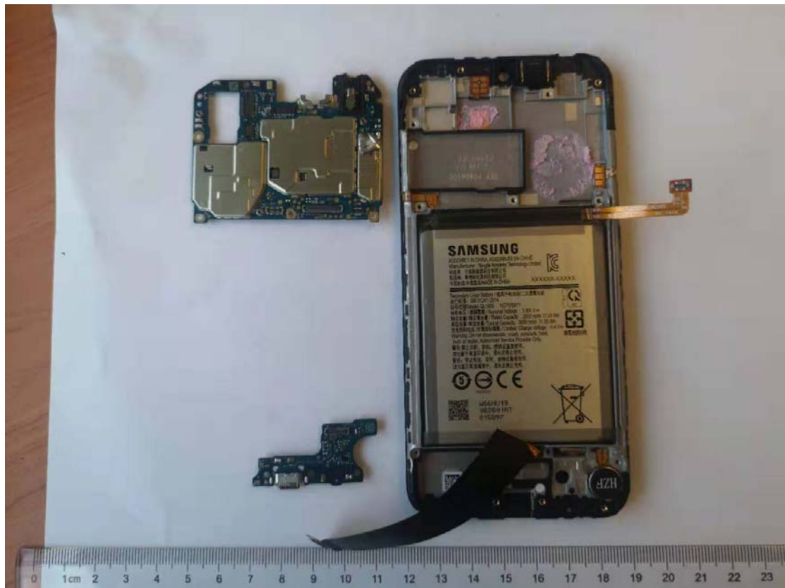
PCB03:
