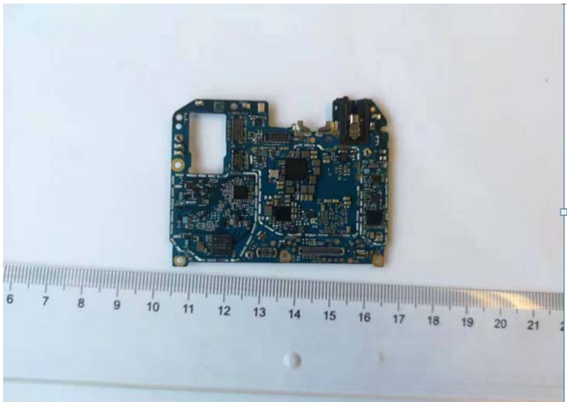
PCB07:
