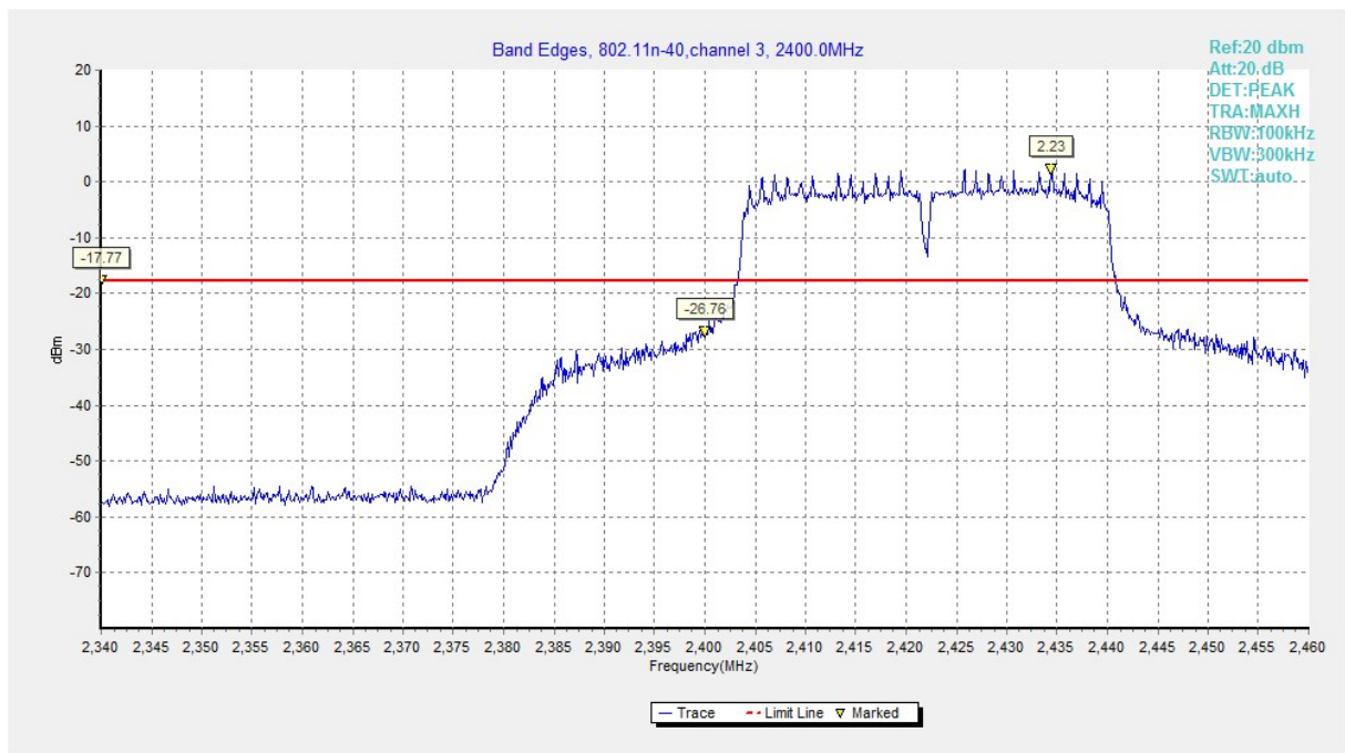
Fig.A.5.7 Band Edges (802.11n-HT40, Ch 3)
