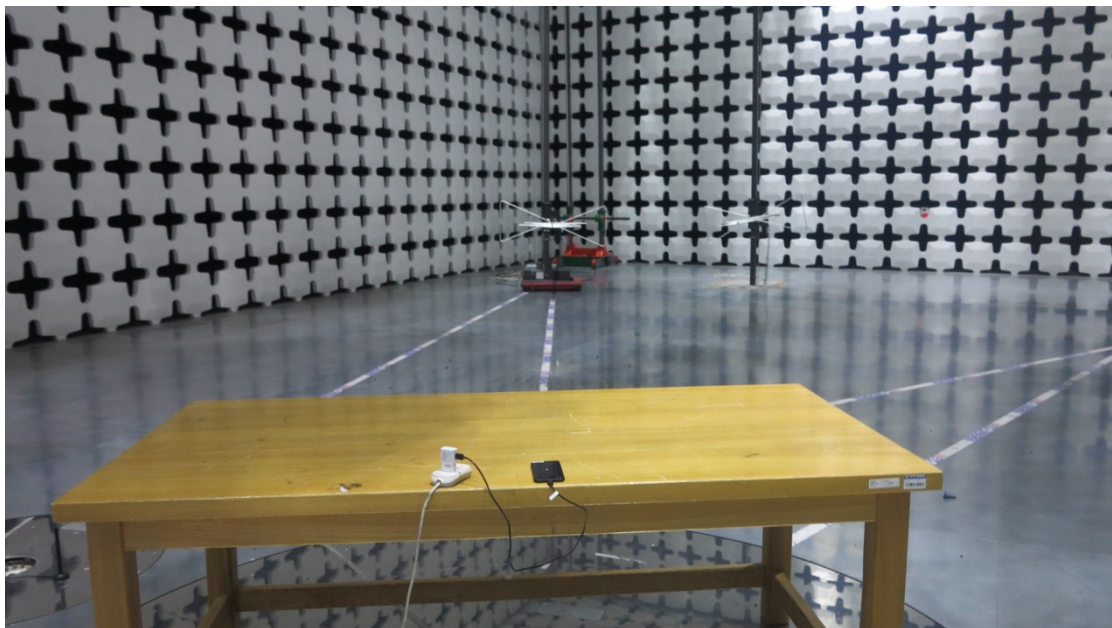
Part 15C: RE: 30M-1GHz
