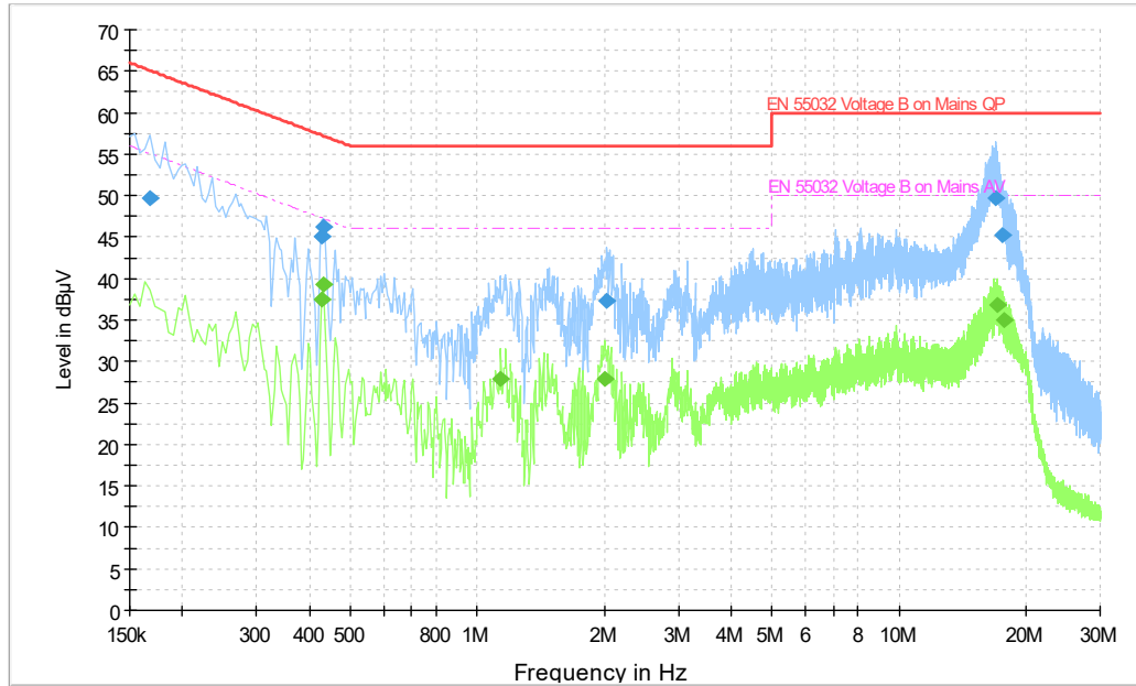
Fig.A.11.1 AC Powerline Conducted Emission- bluetooth
