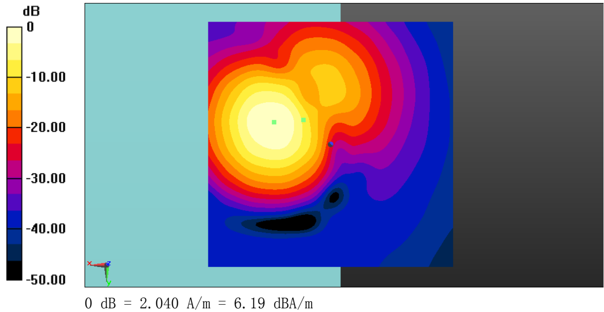
Fig B.16 T-Coil LTE B5
