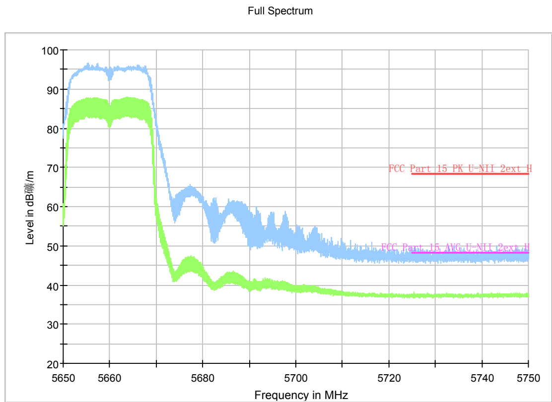
Fig.71 Band Edges (802.11ac-HT40, 5670MHz)
