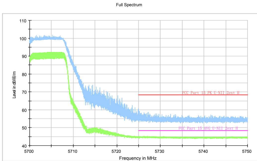
Fig.55 Band Edges (802.11a, 5700MHz)
