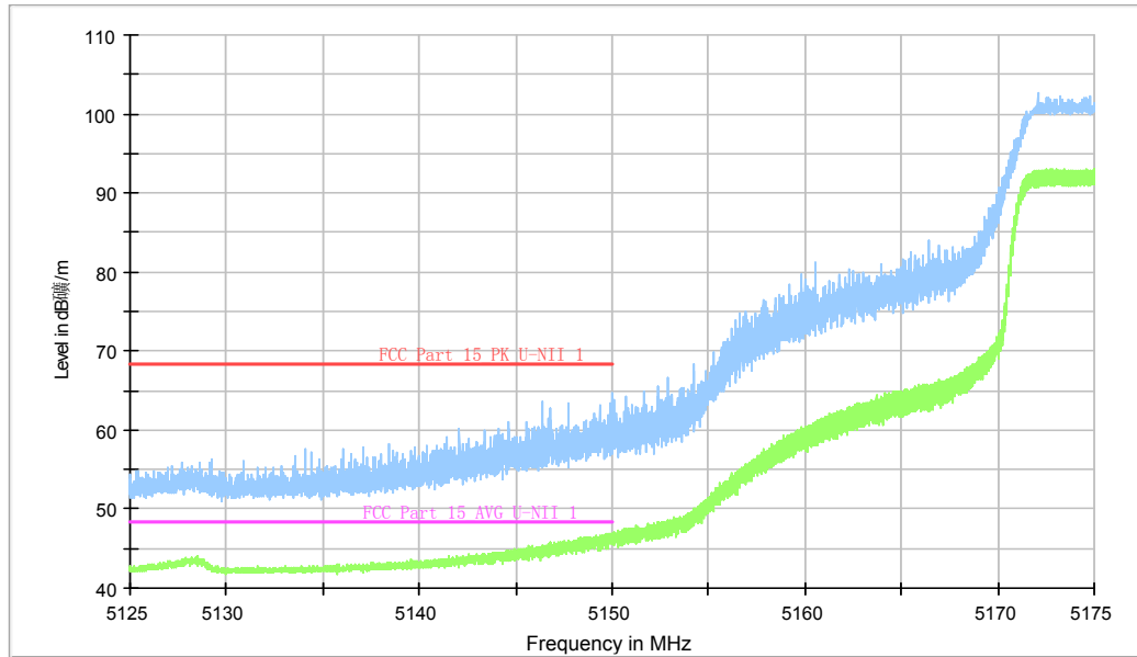
Fig.56 Band Edges (802.11n-HT20, 5180MHz)
