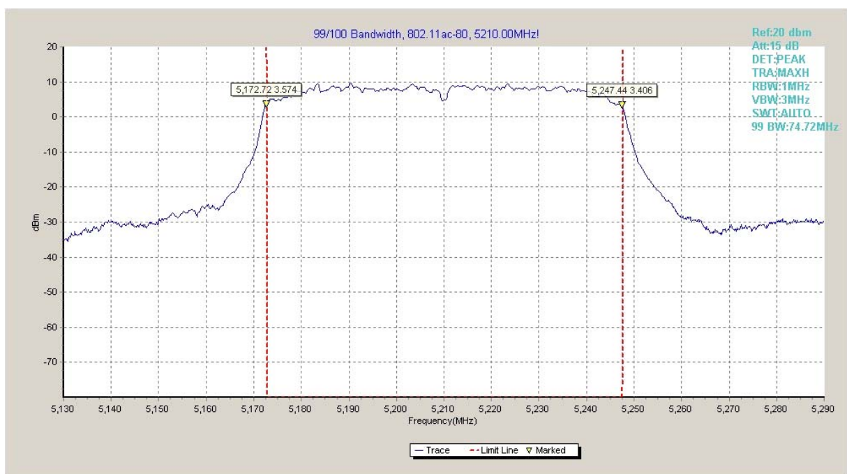
Fig.102 99% Occupied bandwidth (802.11ac-HT80, 5210MHz)
