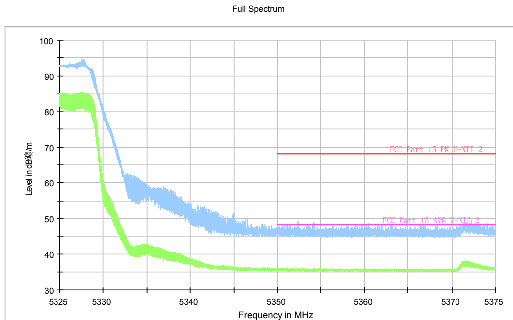
Fig.61 Band Edges (802.11ac-HT20, 5320MHz)
