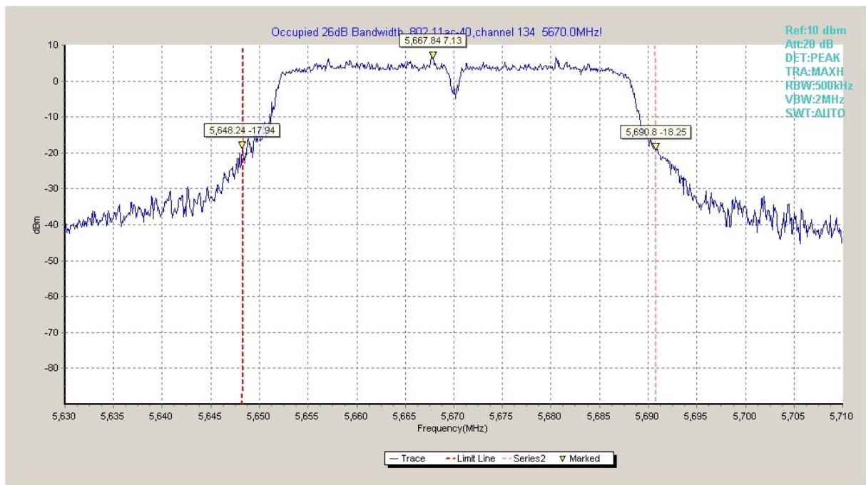
Fig.45 Occupied 26dB Bandwidth (802. 11ac-HT40, 5670MHz)
