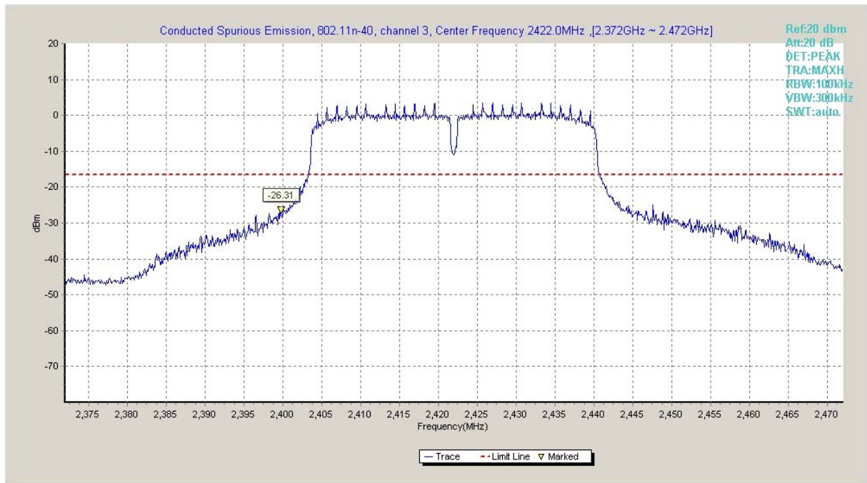
Fig.A.6.1.1 Transmitter Spurious Emission - Conducted (802.11n-HT40, Ch3, Center Frequency)
