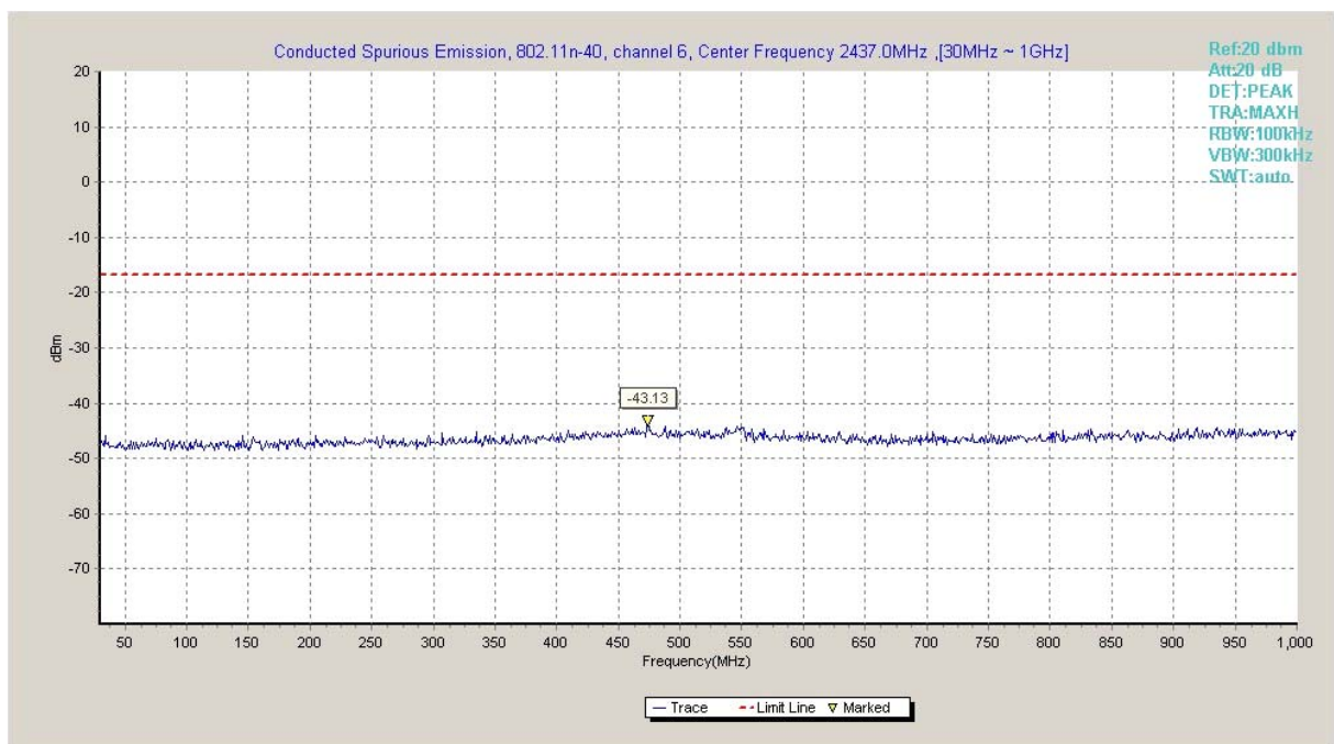
Fig.A.6.1.10 Transmitter Spurious Emission - Conducted (802.11n-HT40, Ch6, 30 MHz-1 GHz)
