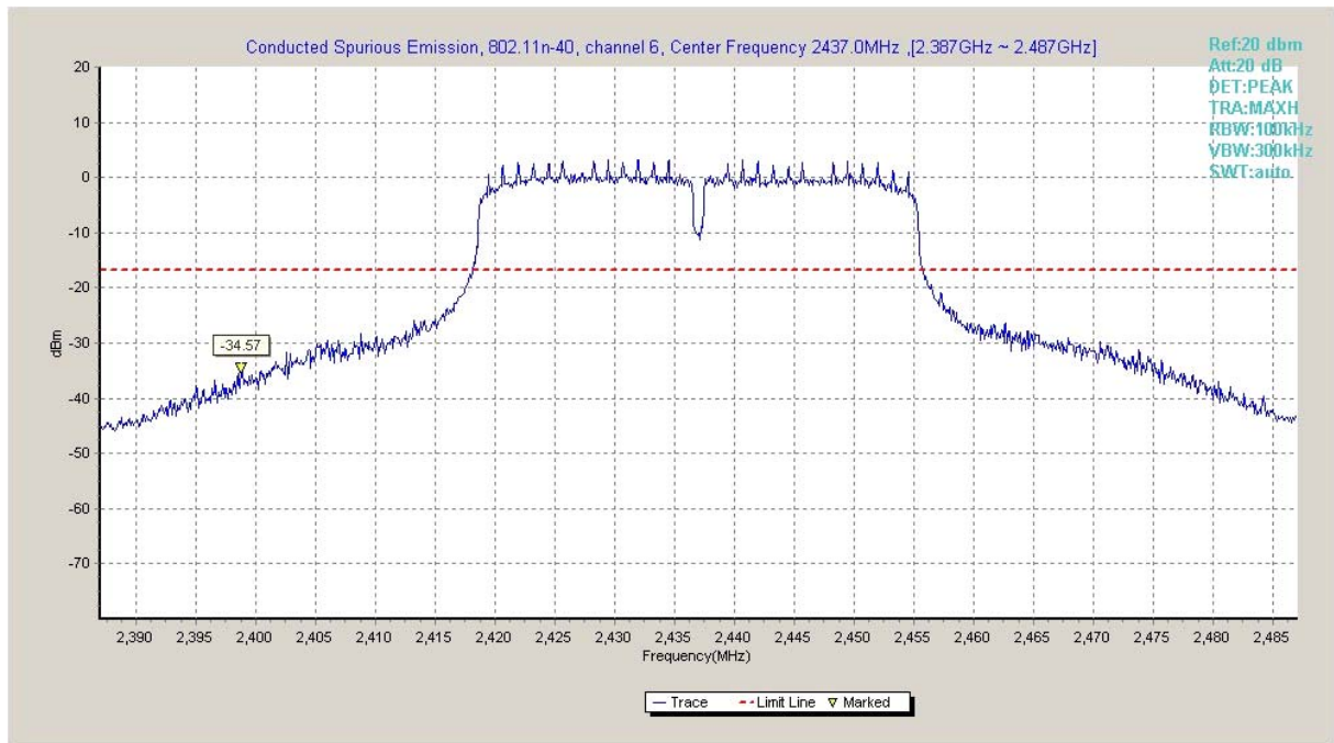
Fig.A.6.1.9 Transmitter Spurious Emission - Conducted (802.11n-HT40, Ch6, Center Frequency)
