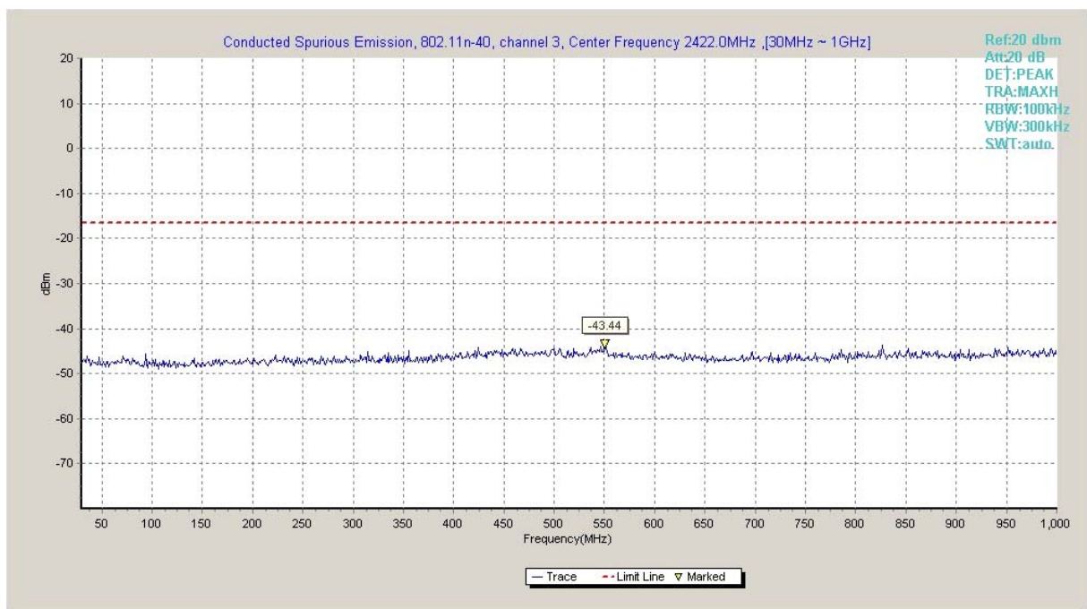
Fig.A.6.1.2 Transmitter Spurious Emission - Conducted (802.11n-HT40, Ch3, 30 MHz-1 GHz)
