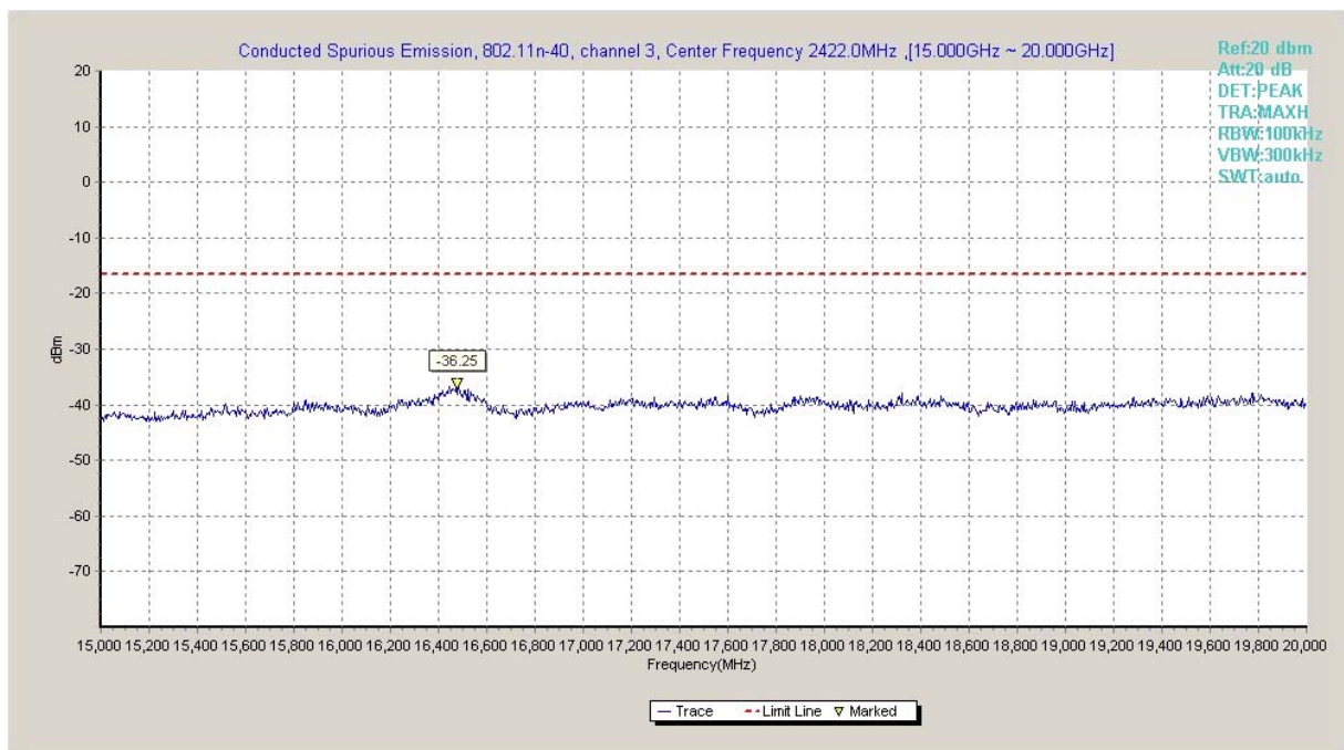
Fig.A.6.1.7 Transmitter Spurious Emission - Conducted (802.11n-HT40, Ch3, 15 GHz-20 GHz)
