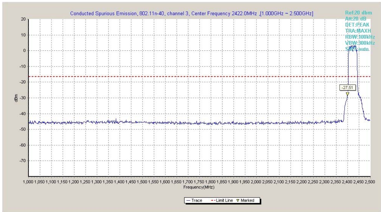
Fig.A.6.1.3 Transmitter Spurious Emission - Conducted (802.11n-HT40, Ch3, 1 GHz-2.5 GHz)
