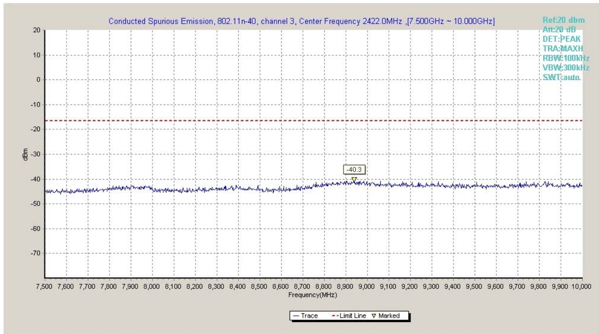
Fig.A.6.1.5 Transmitter Spurious Emission - Conducted (802.11n-HT40, Ch3, 7.5 GHz-10 GHz)
