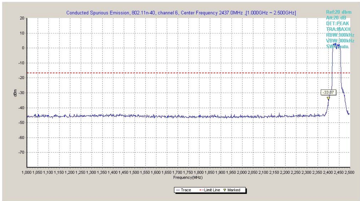
Fig.A.6.1.11 Transmitter Spurious Emission - Conducted (802.11n-HT40, Ch6, 1 GHz-2.5 GHz)
