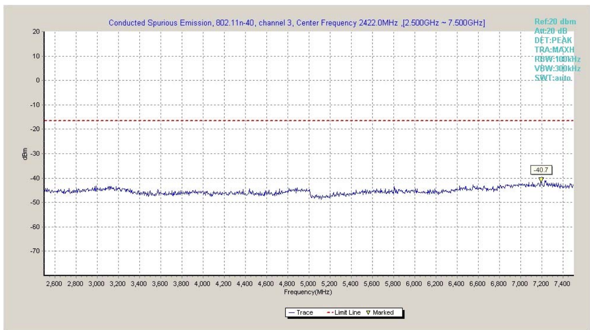
Fig.A.6.1.4 Transmitter Spurious Emission - Conducted (802.11n-HT40, Ch3, 2.5 GHz-7.5 GHz)
