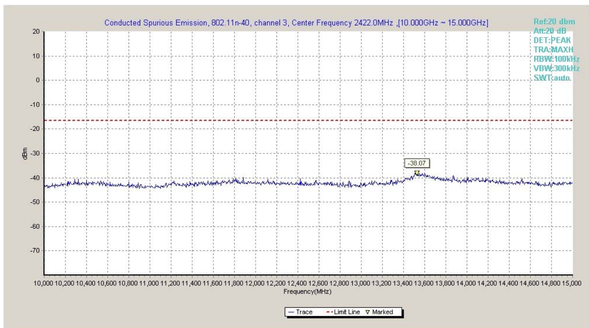
Fig.A.6.1.6 Transmitter Spurious Emission - Conducted (802.11n-HT40, Ch3, 10 GHz-15 GHz)
