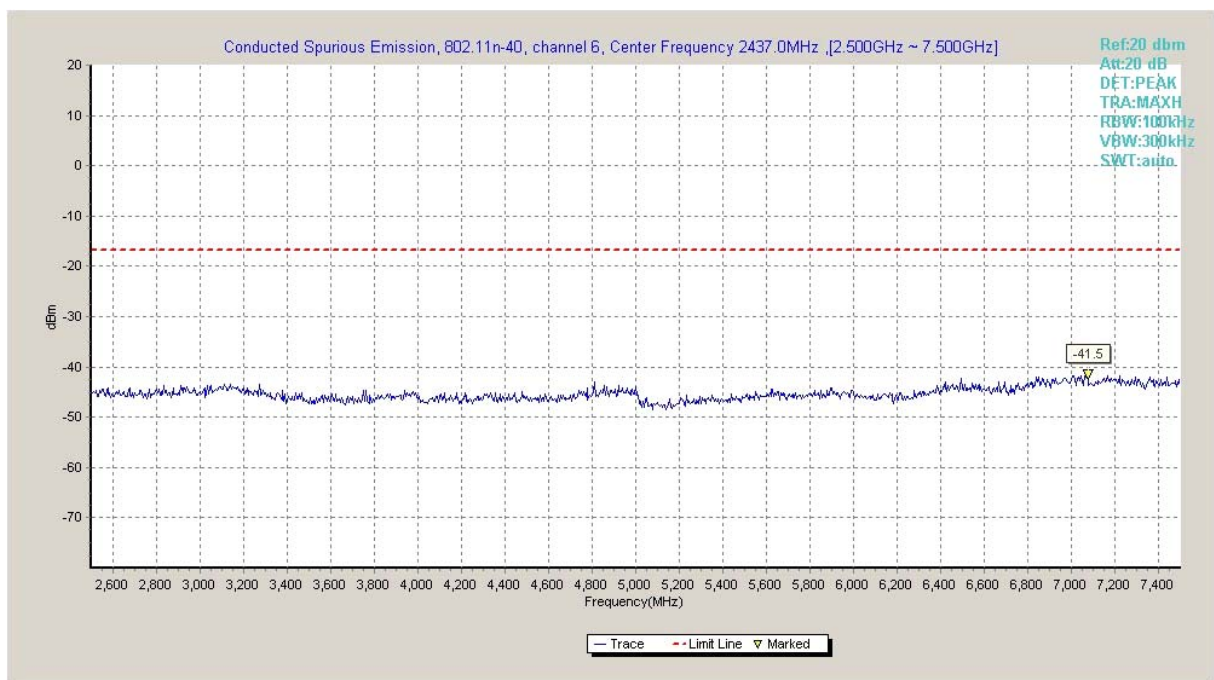
Fig.A.6.1.12 Transmitter Spurious Emission - Conducted (802.11n-HT40, Ch6, 2.5 GHz-7.5 GHz)
