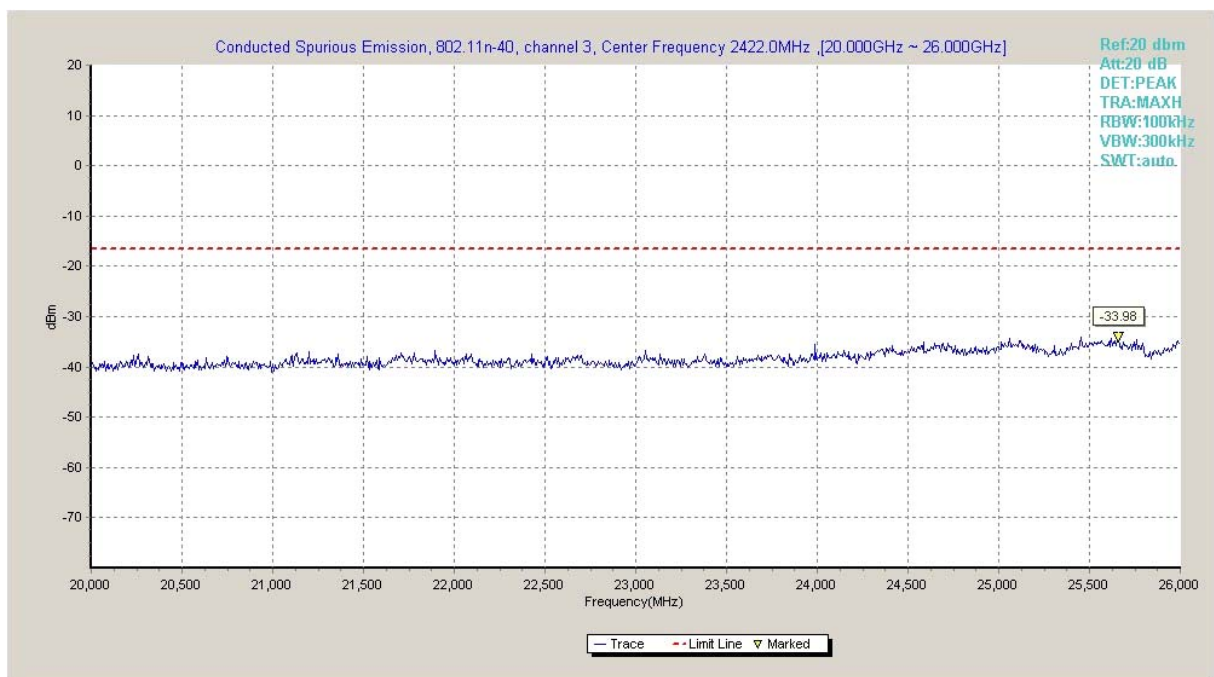
Fig.A.6.1.8 Transmitter Spurious Emission - Conducted (802.11n-HT40, Ch3, 20 GHz-26 GHz)
