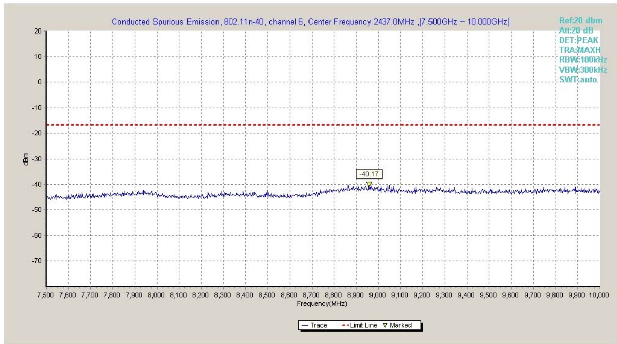
Fig.A.6.1.13 Transmitter Spurious Emission - Conducted (802.11n-HT40, Ch6, 7.5 GHz-10 GHz)
