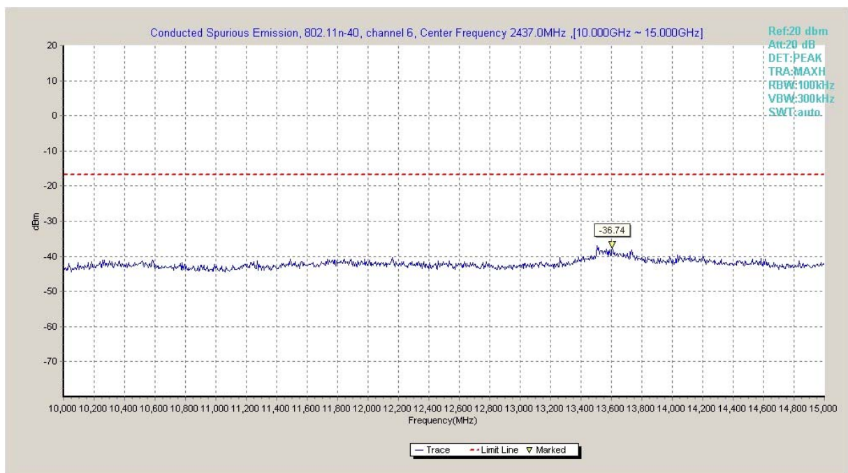
Fig.A.6.1.14 Transmitter Spurious Emission - Conducted (802.11n-HT40, Ch6, 10 GHz-15 GHz)
