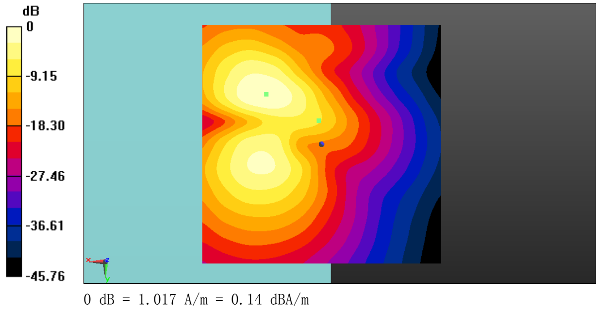
Fig B.11 T-Coil LTE B2
