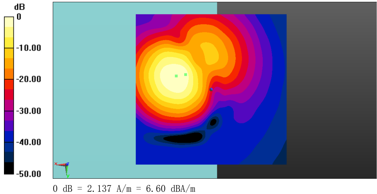
Fig B.20 T-Coil LTE B14
