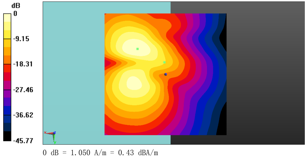
Fig B.17 T-Coil LTE B12
