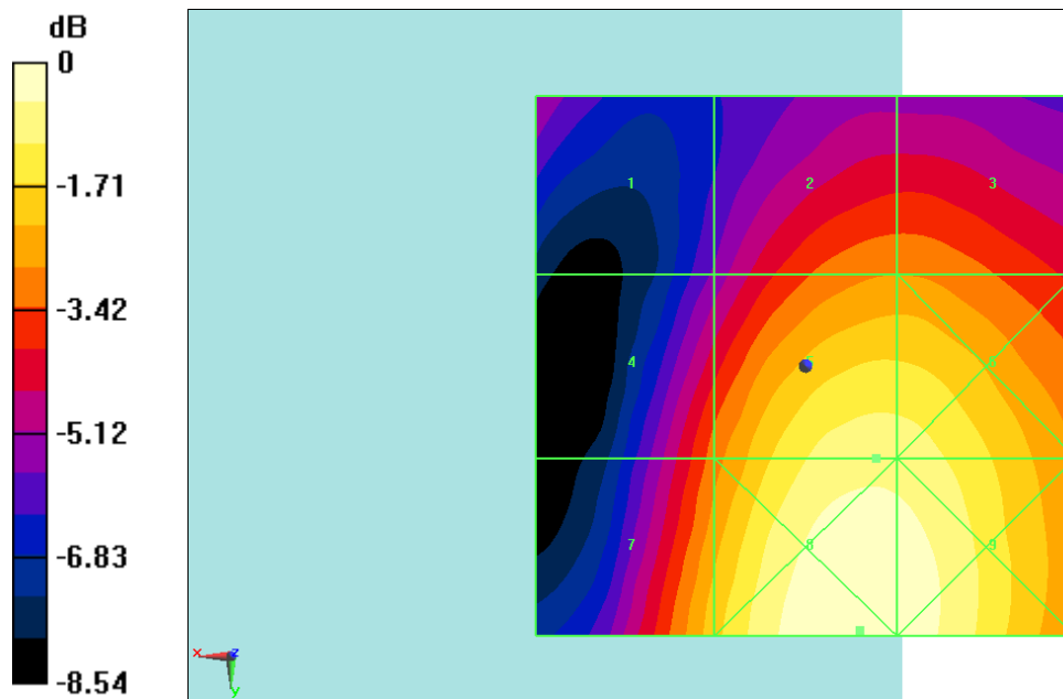
Fig B.5 HAC RF E-Field GSM 1900 Middle
