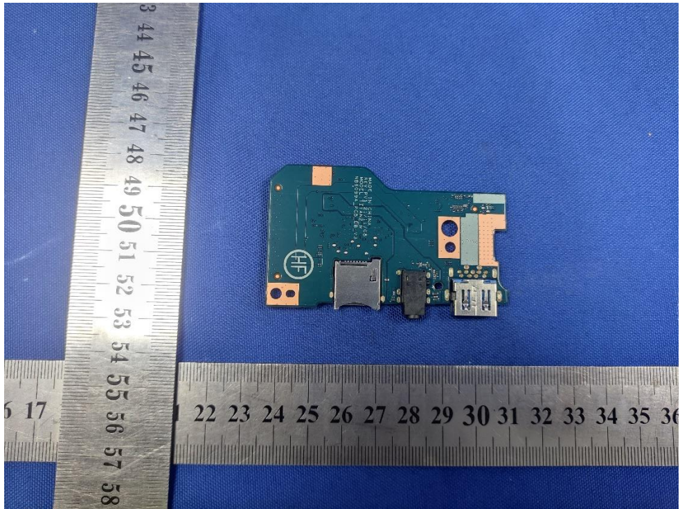
PWB view
