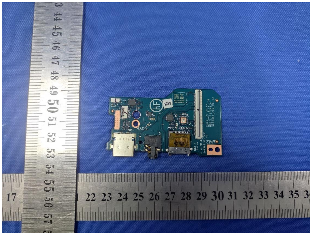
PWB view
