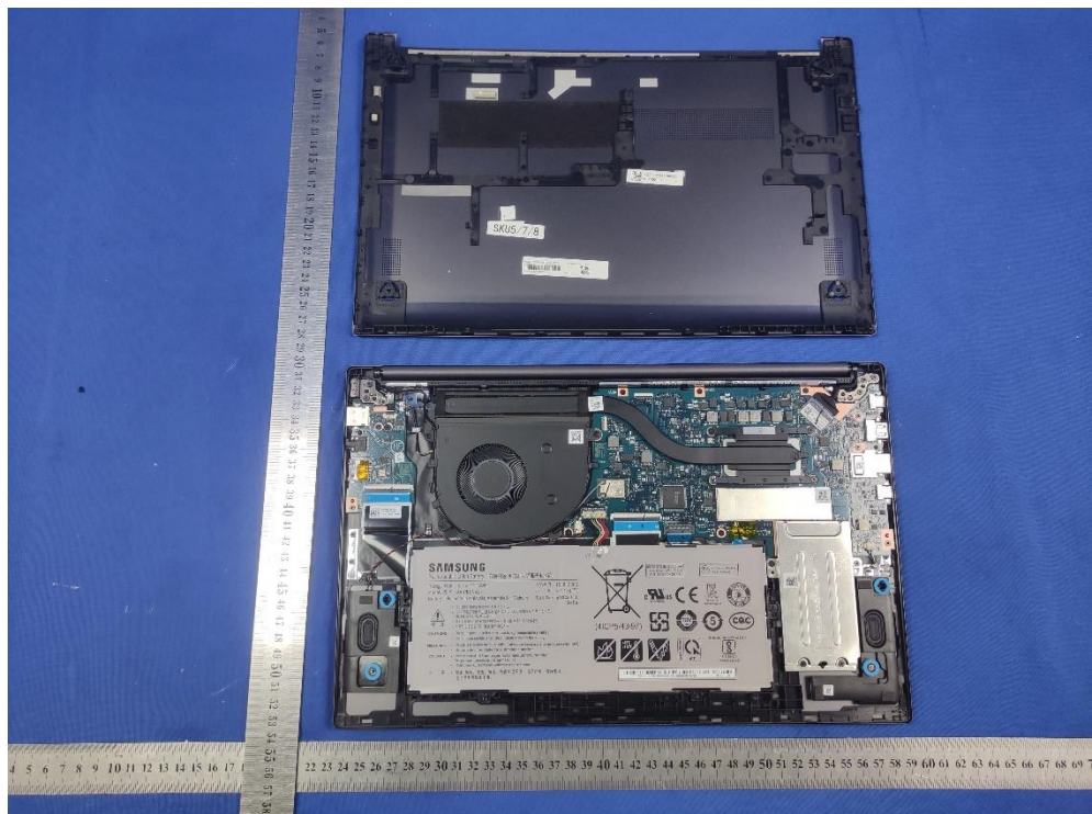
Overall view
