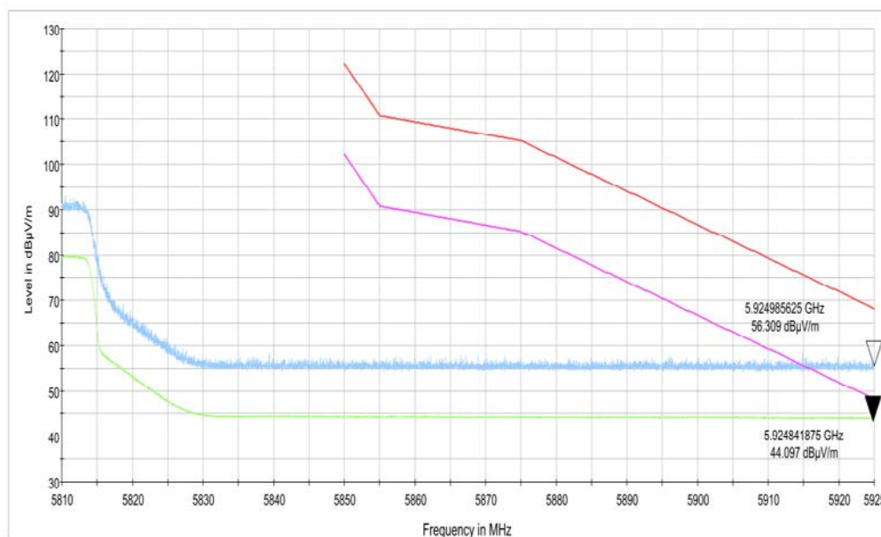
Fig. 36 Band Edges (802.11ax-HT80, CH155, 5775MHz)
