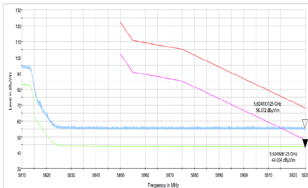
Fig. 34 Band Edges (802.11ax-HT40,CH159, 5795MHz)
