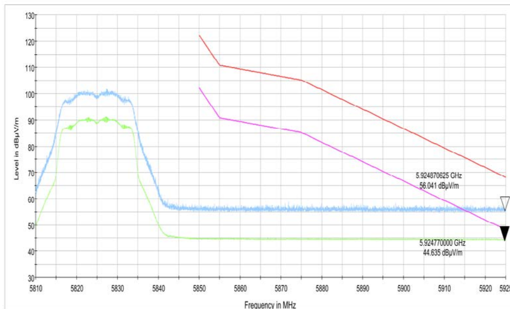
Fig. 26 Band Edges (802.11ac-HT20, CH165, 5825MHz)
