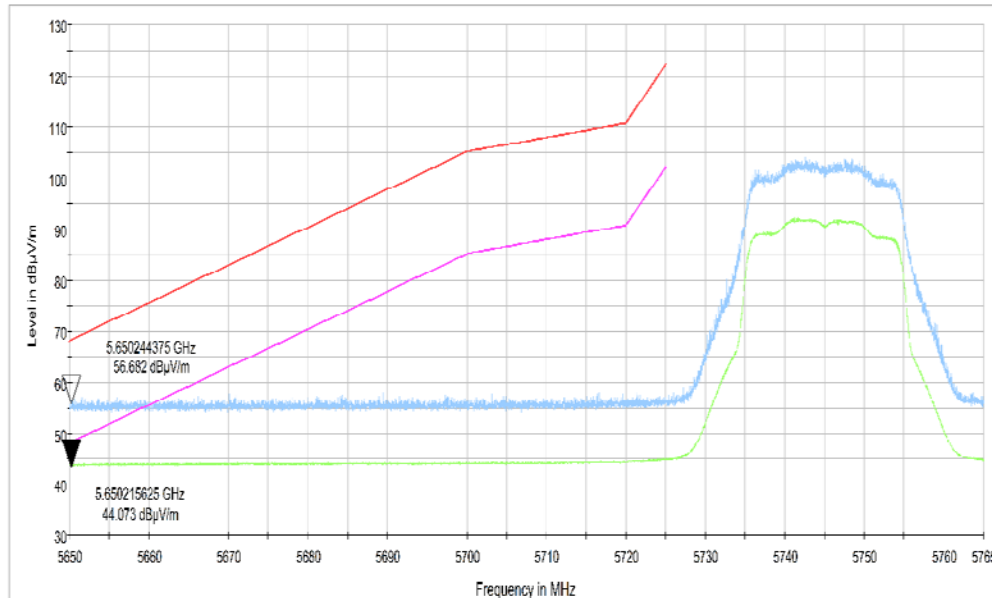
Fig. 31 Band Edges (802.11ax-HT20, CH149, 5745MHz)
