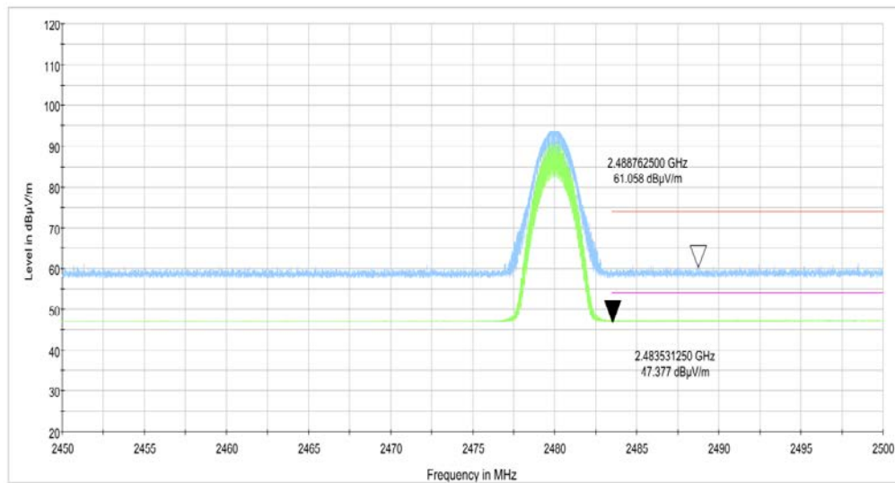
Fig.10. Frequency Band Edges: \pi/4 DQPSK, Channel 78, Hopping Off, 2.45 GHz - 2.50GHz
