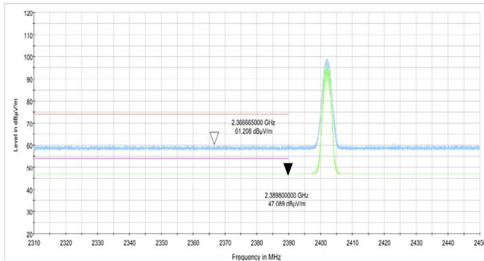
Fig.11. Frequency Band Edges: 8DPSK, Channel 0, 2.31 GHz - 2.45GHz
