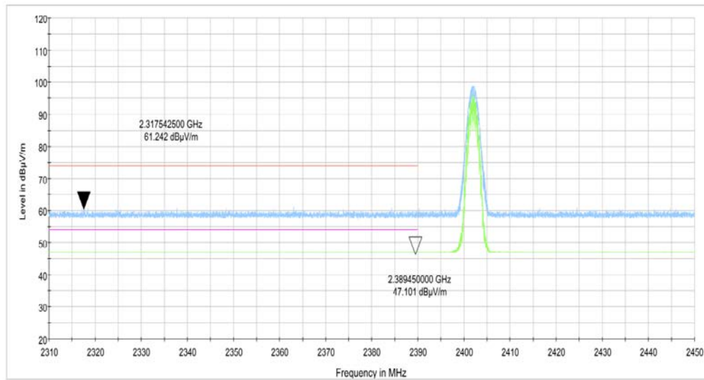
Fig.9. Frequency Band Edges: \pi/4 DQPSK, Channel 0, Hopping Off, 2.31 GHz - 2.45GHz
