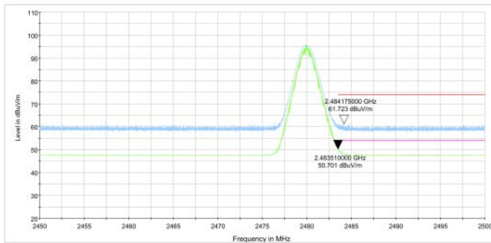
Fig.2. Frequency Band Edges: GFSK, Channel 78, 2.45 GHz - 2.50GHz
