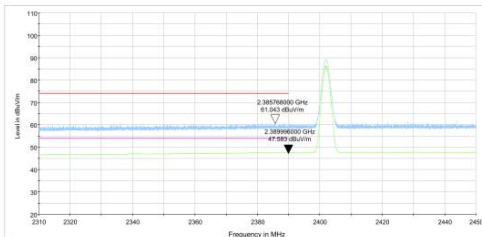
Fig.3. Frequency Band Edges: \pi/4 DQPSK, Channel 0, H2.31 GHz - 2.45GHz
