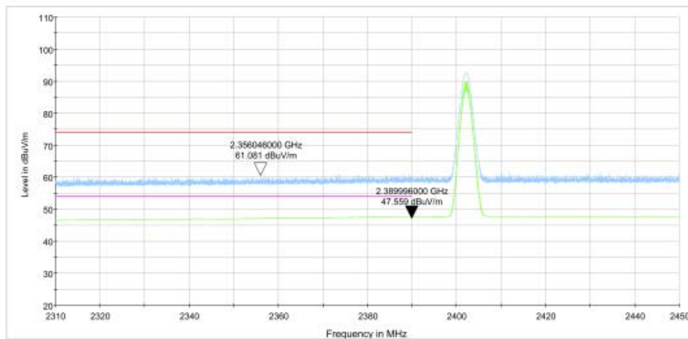
Fig.5. Frequency Band Edges: 8DPSK, Channel 0, 2.31 GHz - 2.45GHz
