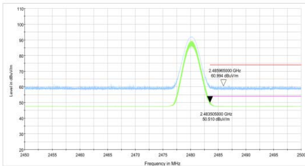
Fig.6. Frequency Band Edges: 8DPSK, Channel 78, 2.45 GHz - 2.50GHz
