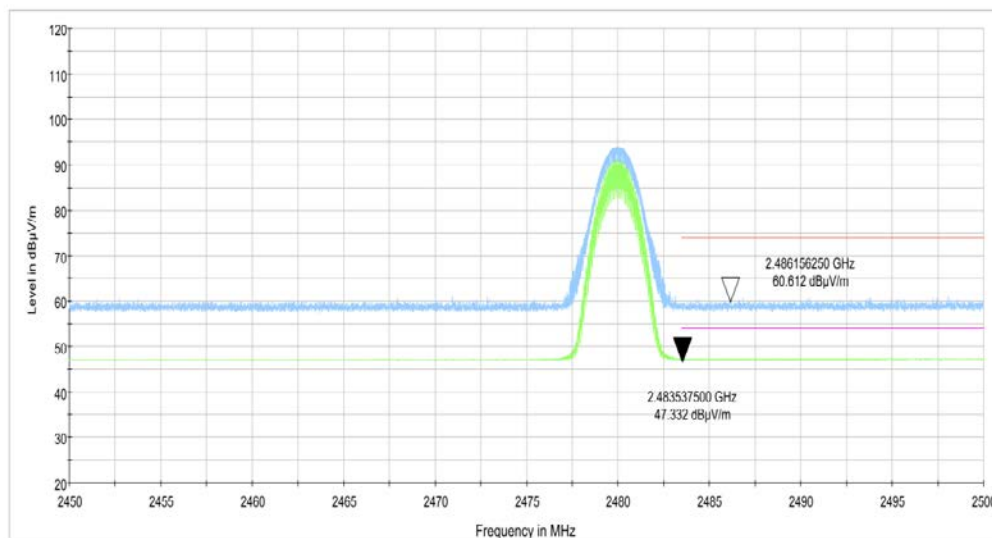
Fig.12. Frequency Band Edges: 8DPSK, Channel 78, 2.45 GHz - 2.50GHz
