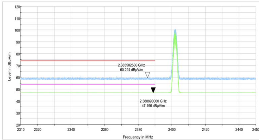
Fig.7. Frequency Band Edges: GFSK, Channel 0, Hopping Off, 2.31 GHz – 2.45GHz
