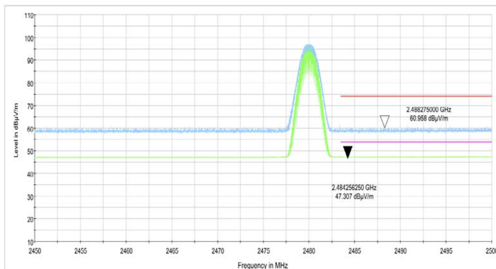
Fig.8. Frequency Band Edges: GFSK, Channel 78, Hopping Off, 2.45 GHz - 2.50GHz
