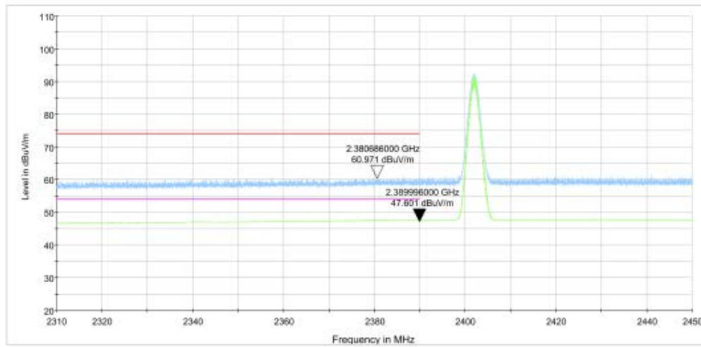
Fig.1. Frequency Band Edges: GFSK, Channel 0, 2.31 GHz – 2.45GHz
