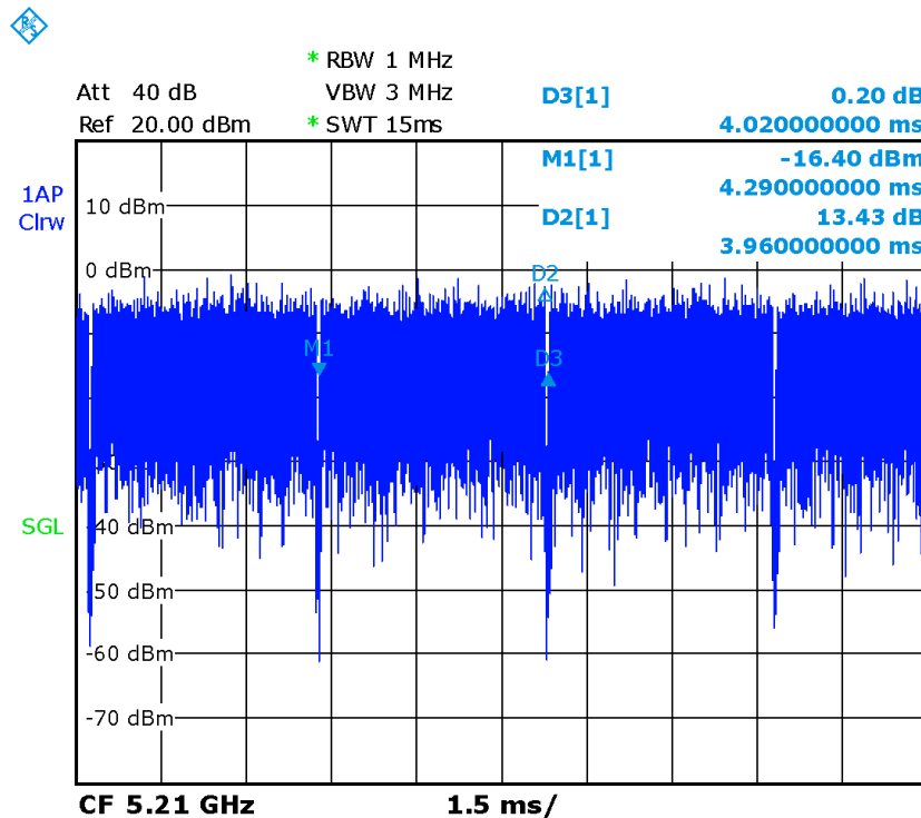
Picture 13.5 Duty factor plot for 5G
