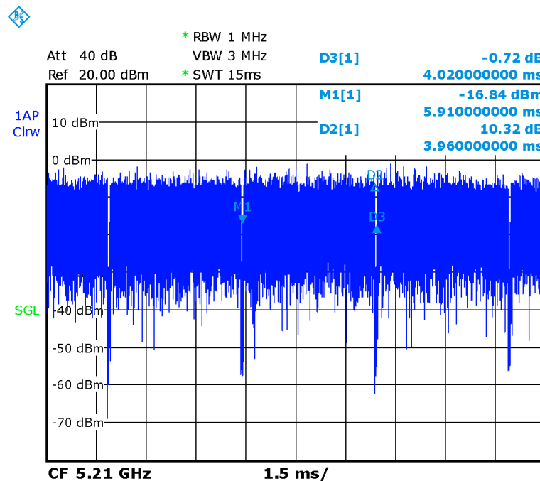
Picture 13.4 Duty factor plot for 5G
