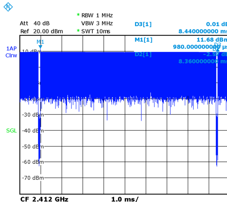
Picture 13.1 Duty factor plot for 2.4G
