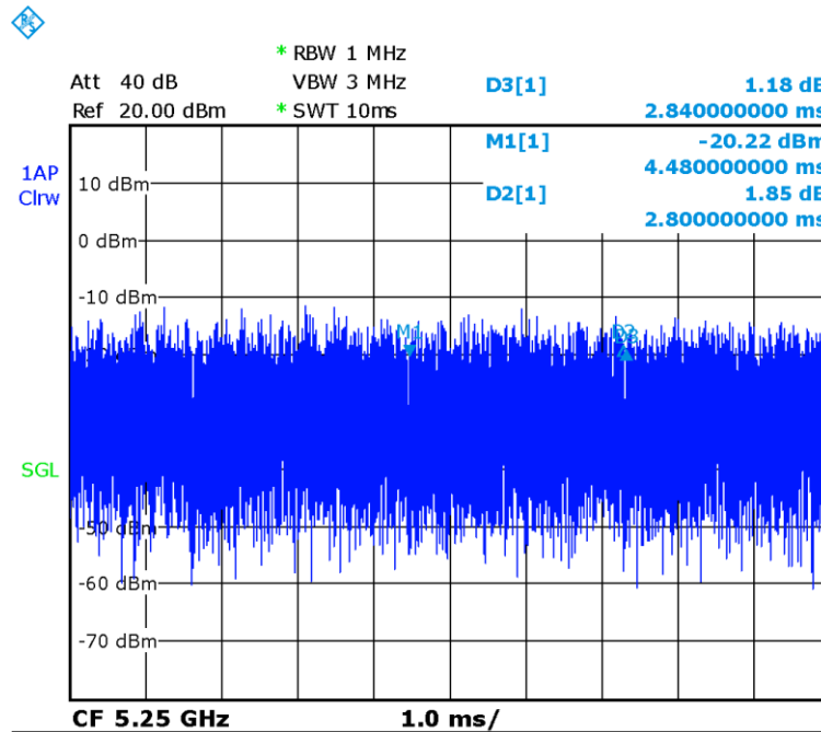
Picture 13.6 Duty factor plot for 5G
