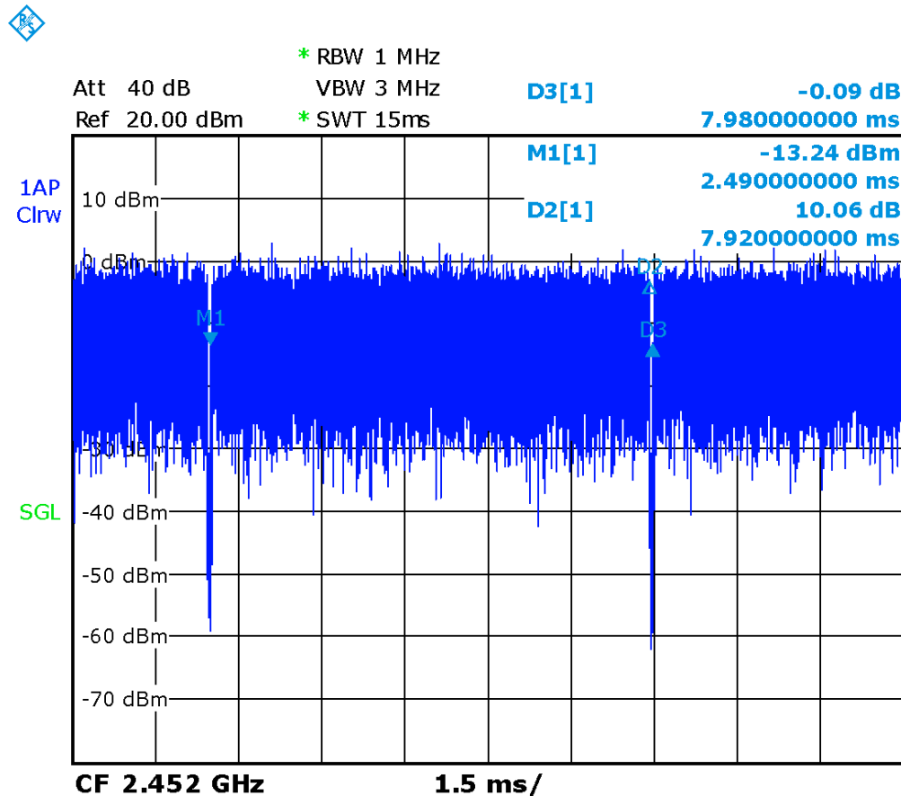
Picture 13.3 Duty factor plot for 2.4G
