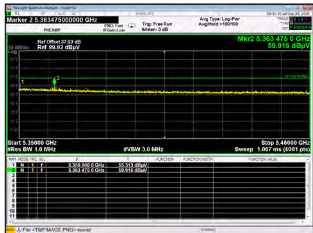
U-NII-2A 11ax80 CH58 Peak
