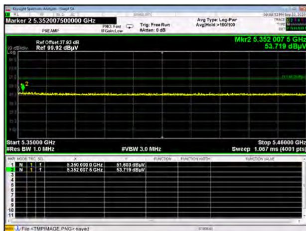
U-NII-2A 11ax40 CH62 Peak
