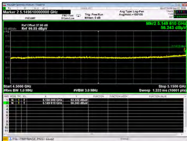
U-NII-1 11ac160 CH50 Peak
