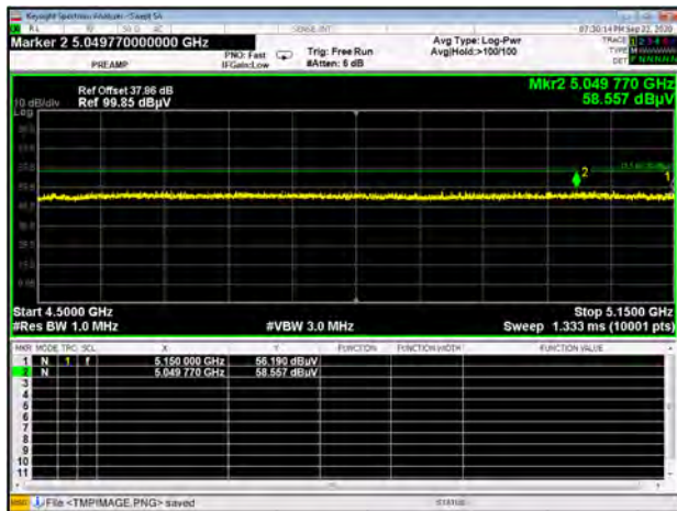
U-NII-1 11ax20 CH36 Peak
