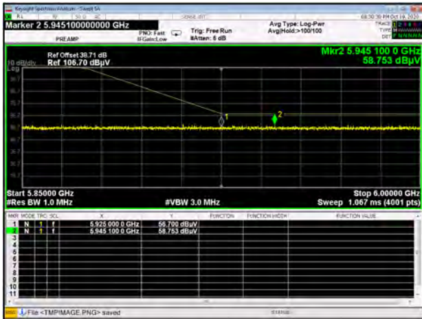
U-NII-3 11ac20 CH144 Peak
