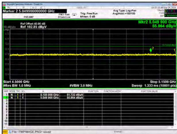
U-NII-1 11ax40 CH38 Peak
