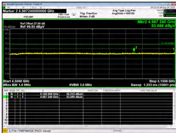
U-NII-2A 11ax40 CH54 Peak
