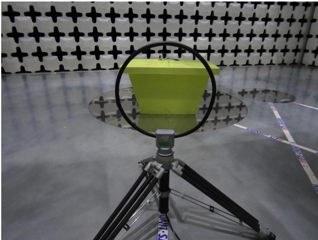
Occupied Bandwidth and Radiated emission (9kHz-30MHz)
