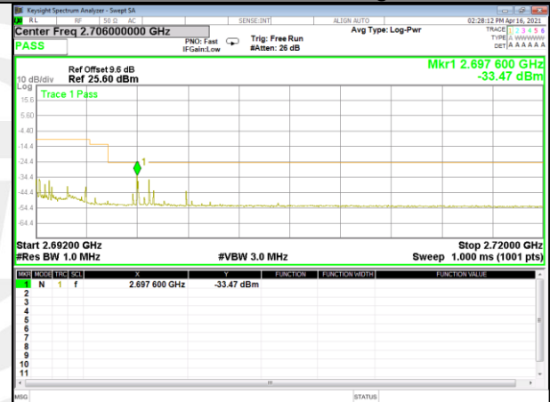
Band 41_5M_16QAM_High_1-RB
