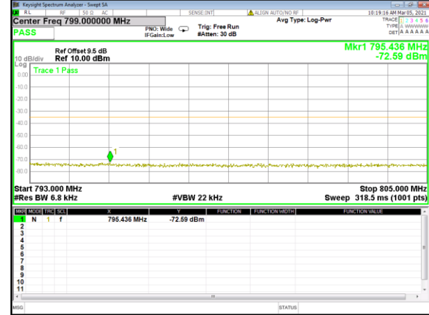
Band 13_5M_16QAM_High_Full-RB
