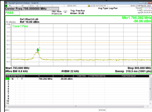
Band 13_10M_QPSK_High_Full-RB
