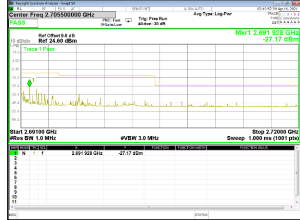
Band 41_15M_16QAM_High_Full-RB
