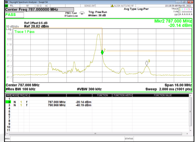
Band 13_5M_16QAM_High_Full-RB
