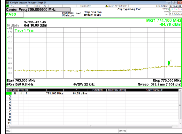
Band 13_10M_QPSK_High_1-RB
