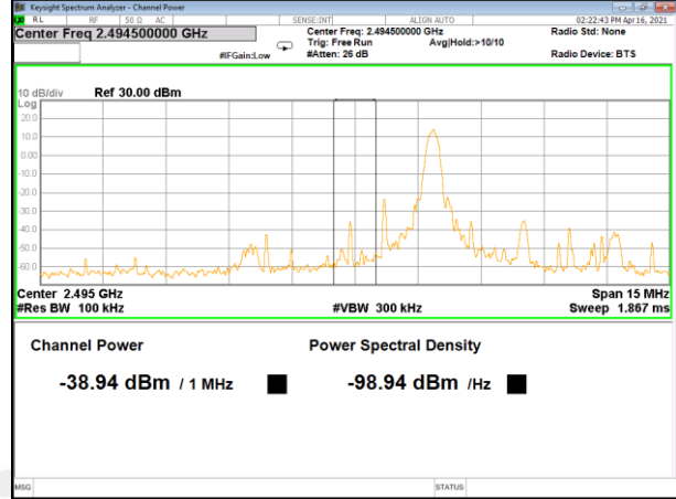
Band 41_5M_QPSK_Low_Full-RB
