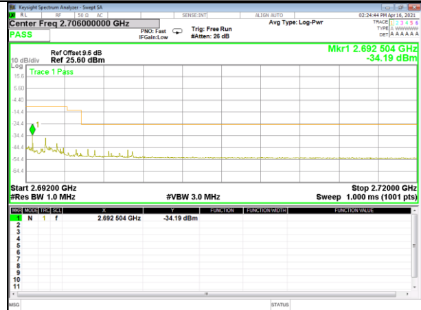
Band 41_5M_QPSK_High_1-RB
