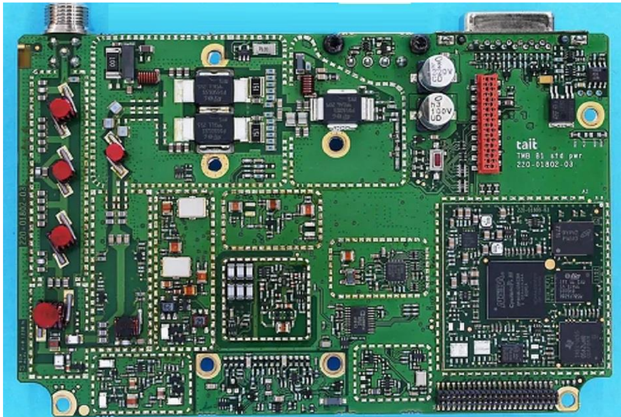
16202005_Top view (with and without cans)
