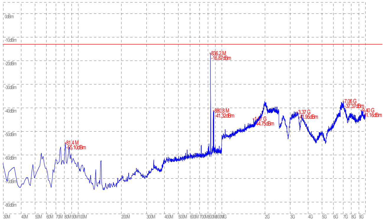
(Plot A.4: GSM 850MHz Channel = 190, Test Antenna Vertical)
