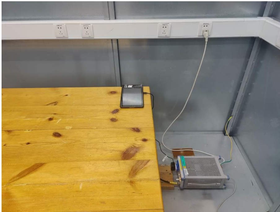
14. Conducted Emission (Part 15B, Camera)
