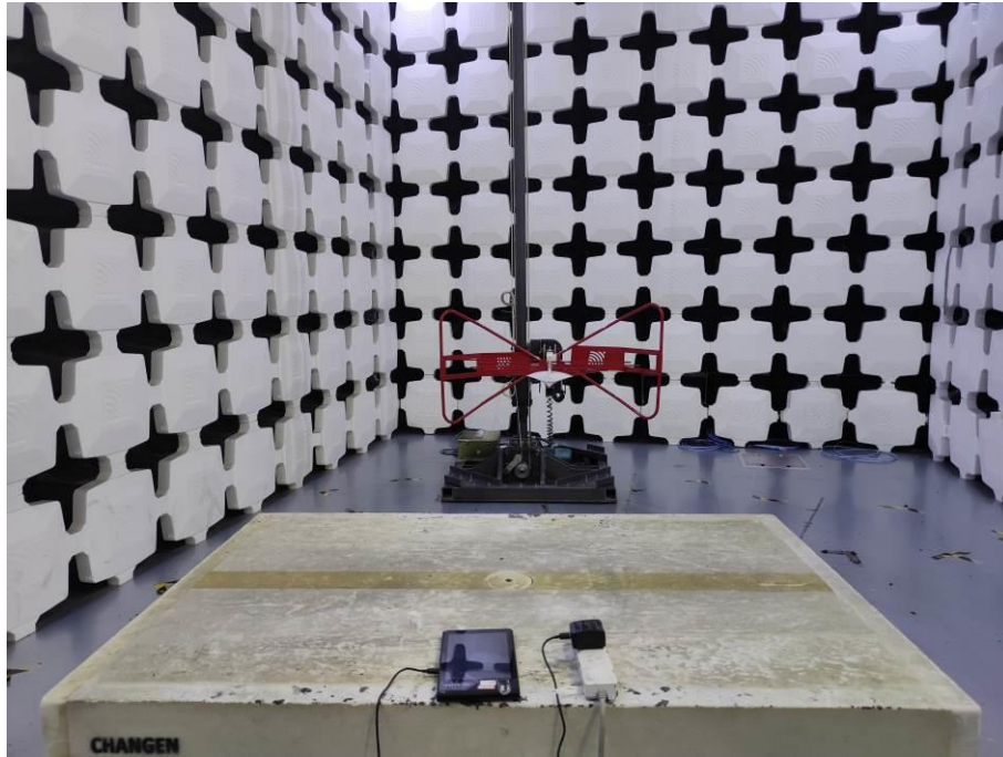
9. Radiated Emissions (Part 15B, Camera, 30MHz-1GHz)
