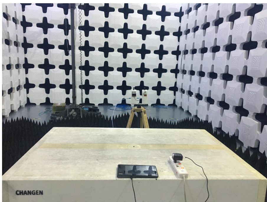
7. Radiated Emissions (Part 15B Charging Mode,26.5GHz-40GHz)
