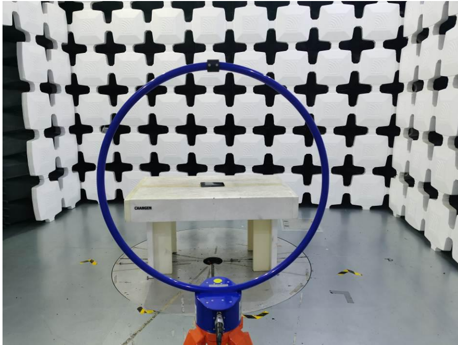
9. Radiated Emissions (Part 15C&Part 15E, 9kHz-30MHz)
